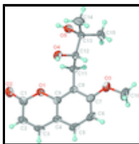
Fig. 1. Anisotropic displacement ellipsoid plot (Barbour, 2001) of \text{C}_{15}\text{H}_{18}\text{O}_5 ; at the 50% probability level; hydrogen atoms are drawn as spheres of arbitrary radius.
