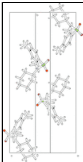
Fig. 2. Unit cell packing for (I).
