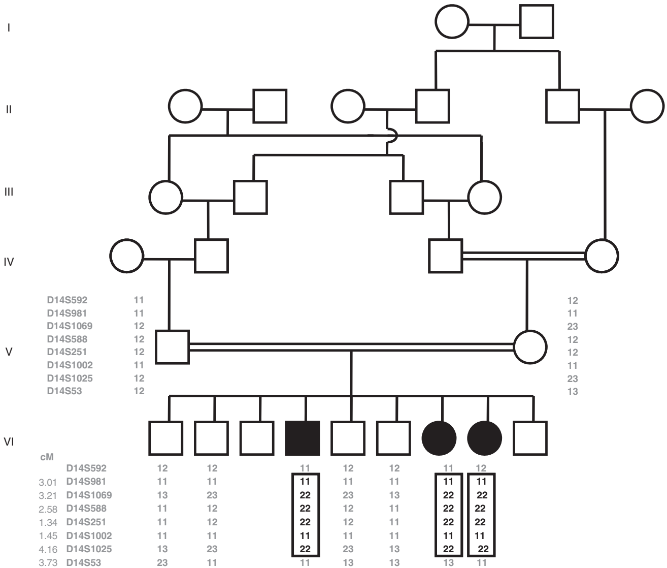
Figure 2 Linkage analysis in family 1. The parents were second cousins. The 14q linkage region was initially identified by a genome-wide 10K GeneChip microarray of SNPs in three affected siblings, then further analyzed by microsatellite polymorphisms in affected and unaffected siblings and parents, as shown. A single linkage region was found where all patients and no unaffected siblings were homozygous, yielding a maximal multipoint LOD score of 2.87 at D14S1002.
