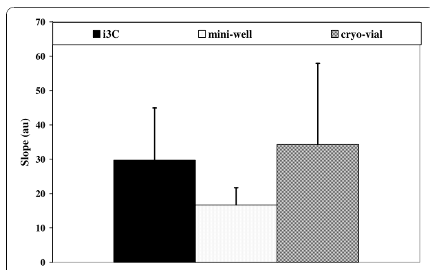
Figure 7 Fluorescein diacetate hydrolysis rates at 19 hours after thawing. For the evaluation of the metabolic recovery after the freezing - thawing cycle, the cells were stained by FDA and the linear slope FI(t) was calculated for each single cell by image analysis. The mean slopes for U937 cell groups that underwent the freezing - thawing cycle in the cryo-devices (at least 4 experiments for each cryo-device) are presented as mean \pm SD.
