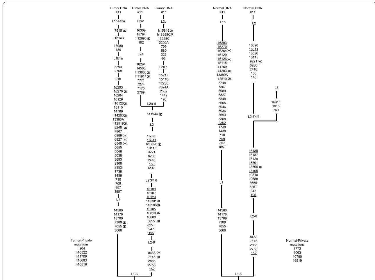
Figure 2 The phylogenetic reconstruction of the sessile serrated adenoma (SSA) case 11 mtDNA sequence from Sui et al. [2]. For additional information, see the fig. 1 legend.
