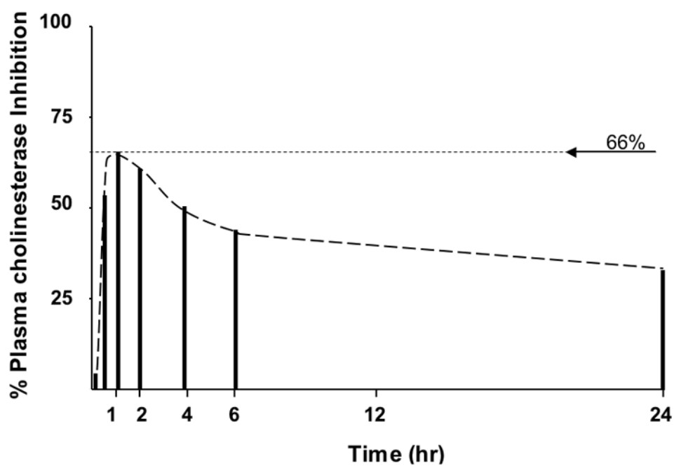
Figure 2. Time-dependent plasma cholinesterase inhibition following a single intraperitoneal dose of compound 16 in rat.
