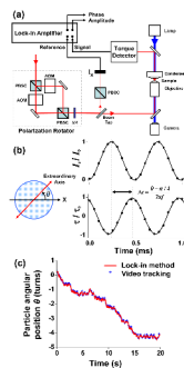
Figure 1. Method of constant optical torque generation and angular position detection. (a) Simplified schematic of the passive optical torque wrench. The optical setup is similar to what has been previously described [6] but with the important addition of a lock-in amplifier. (b) The lock-in amplifier uses I_x(t) as reference signal and the torque detector signal \tau(t) as the input signal. The phase difference between these two signals provides the angular position \theta of the cylinder. (c) Comparison of detected angular position of a quartz dust particle as simultaneously determined by the lock-in method (red line) and video tracking method (blue points). For both (b) and (c), f_{\text{critical}} = 9 \text{ Hz} and f = 1 \text{ kHz} .
