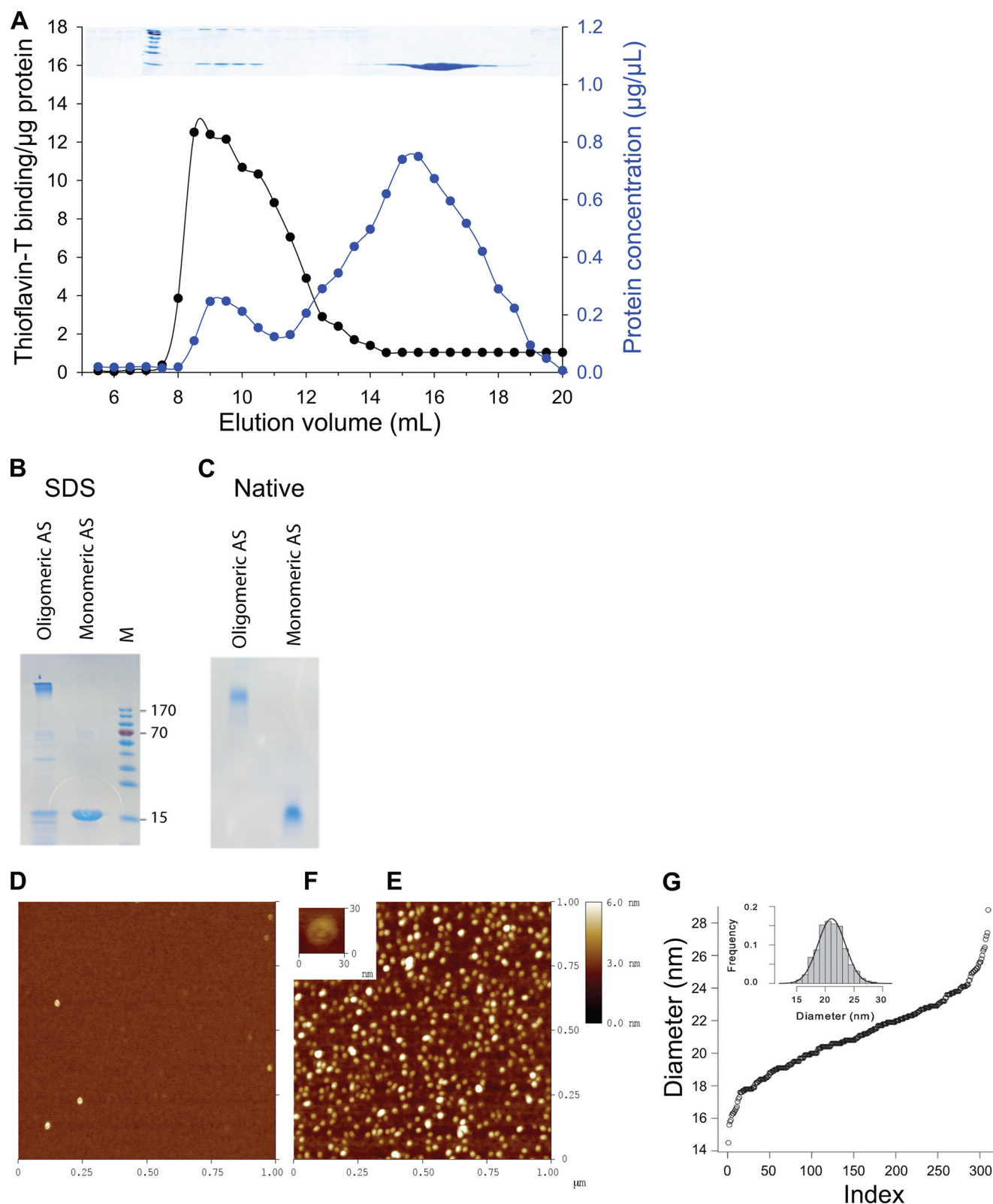
FIGURE 2. Characterization of recombinant human \alpha -synuclein (AS). A , shown is size exclusion chromatography of recombinant \alpha -synuclein from the resolubilized ammonium sulfate pellet of the heat-treated crude extract shown in lane 3 of Fig. 1, A and B . Elution profile from the Superose 6 column shows the protein concentration profile according to the absorbance at 280 nm (blue circles) and the Th-T fluorescence profile (black circles). Above the inset , Coomassie stain of the corresponding eluted fractions after separation on 12% SDS-PAGE is shown. B and C , two fractions were pooled from 15–18 ml as monomeric AS and from 7.5–11 ml as oligomeric AS, concentrated, and further separated by SDS-PAGE ( B ) or native-PAGE ( C ) and Coomassie-stained. Standard molecular masses ( M ) in kDa are indicated for the SDS-gel. D–F , shown are atomic force microscopy morphological studies of AS monomers and AS oligomers, as in B and C . Atomic force microscopy images ( 1 \mu\text{m} \times 1 \mu\text{m} ) of AS monomers ( D ) and AS oligomers ( E ) are shown. At higher magnification, AS oligomers present a globular flattened-shape structure ( F ). G , shown is cumulative function of the diameter distribution of the AS oligomers with a mean size of 21.1 nm and a S.D. s = 2.4 nm. Inset , shown is s histogram of the distribution superimposed with a Gaussian (mean = 21.1 nm, s = 2.4 nm).
