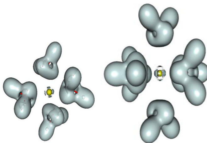
Figure 3. ELF localization domains (basins) for the \text{Zn}^{2+}\text{-(H}_2\text{O)}_4 and \text{Zn}^{2+}\text{-(H}_2\text{O)}_6 complexes. Again, non covalent \text{V}(\text{Zn}) basin are observed.
