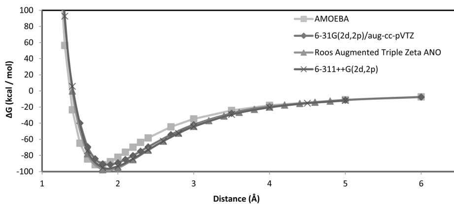
Figure 5. Binding energy of zinc and water dimer in gas phase as a function of separation distance. The 6-31G(2d,2p)/aug-cc-pVTZ indicates that 6-31G(2d,2p) was used to represent the \text{Zn}^{2+} cation and aug-cc-pVTZ was used to represent the water molecule. Binding energy obtained from the last two basis sets used the same basis sets for both ion and water.
