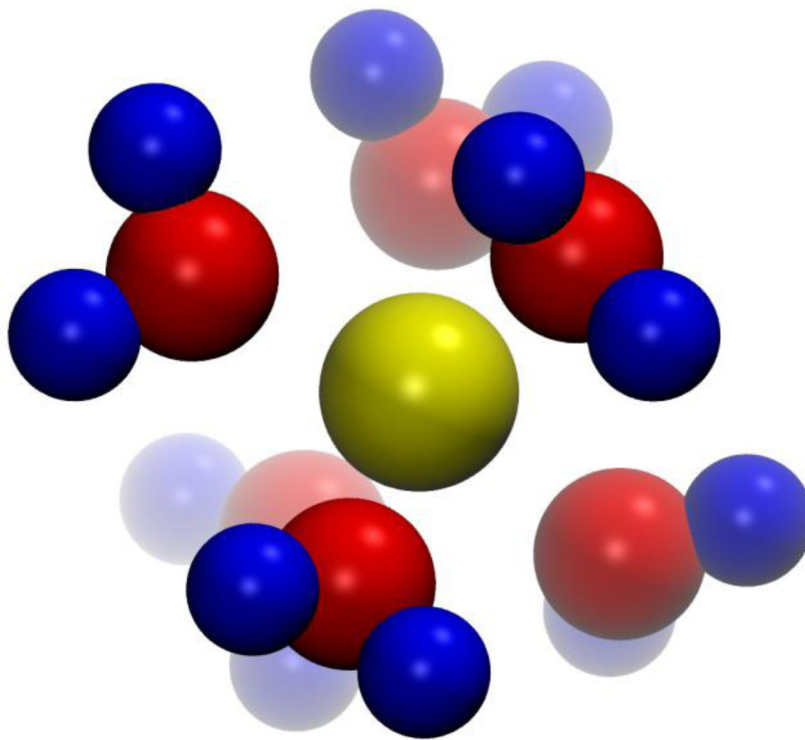
Figure 10. First solvation shell around Zn 2+ ion.
