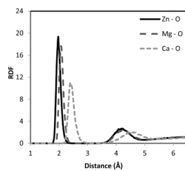
Figure 7. Radial distribution function of divalent cations ( \text{Zn}^{2+} , \text{Mg}^{2+} , and \text{Ca}^{2+} ) and oxygen atom in water.
