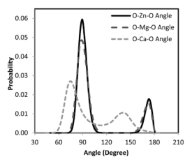
Figure 8. Water-Ion-Water Angle distribution of divalent cations ( \text{Zn}^{2+} , \text{Mg}^{2+} , and \text{Ca}^{2+} ) and oxygen atom in water.
