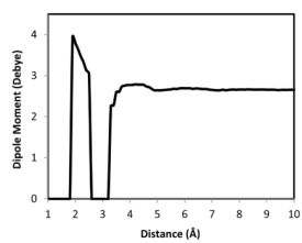
Figure 9. Dipole moment at each distance (Å) around ion.
