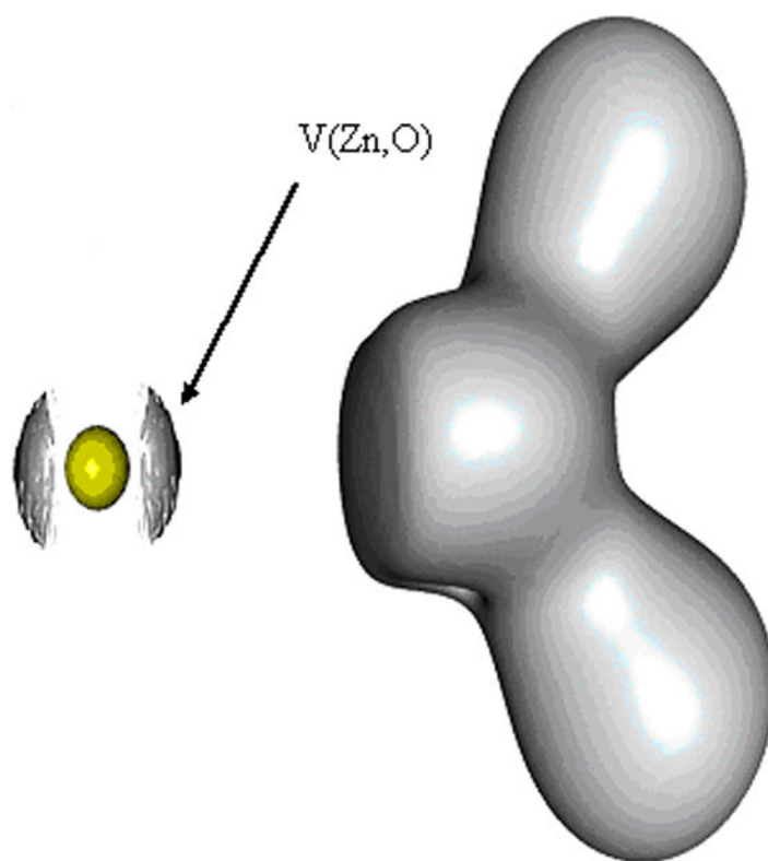
Figure 1. ELF localization domains (basins) for the \text{Zn}^{2+}\text{-H}_2\text{O} complex. A covalent \text{V}(\text{Zn}, \text{O}) basin reflecting electron sharing is observed and reveals the covalent nature of the Zn-O interaction.
