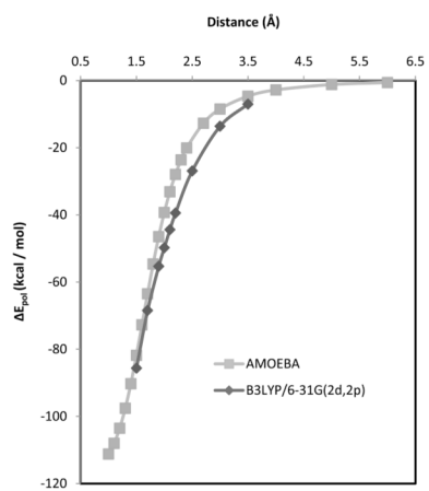
Figure 4. Polarization energy of zinc and water dimer in gas phase as a function of separation distance.
