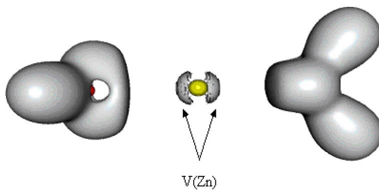
Figure 2. ELF localization domains (basins) for the \text{Zn}^{2+}-(\text{H}_2\text{O})_2 complex. Non-covalent V(\text{Zn}) basin are observed describing the deformation of \text{Zn}^{2+} outer-shells density within the fields of the water molecules.
