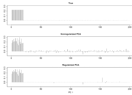
Fig 1. A simulated data set with n = 100 , d = 200 , and k = 1 . Top, middle and bottom panels show respectively the true loadings, loadings from the nonregularized logistic PCA and from the regularized logistic PCA. The penalty parameter is selected using the BIC.
