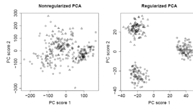
Fig 2. The scatterplots of the first two PC scores from the nonregularized (left) and regularized logistic PCA. Circle, rectangle and triangle represent Caucasian, African and Asian population respectively.
