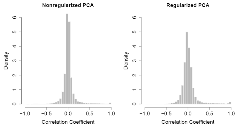
Fig 4. Histograms of pairwise correlations of Pearson's residuals from nonregularized (left) and regularized (right) logistic PCA
