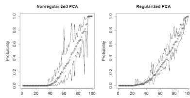
Fig 3. The SNP data: 90% bootstrap variability envelope (showed as lines) of the probability estimates, using 100 randomly selected SNPs. Circles are the estimated probabilities \hat{\pi}_{ij} from the SNP data. Results are based on 100 bootstrap samples.
