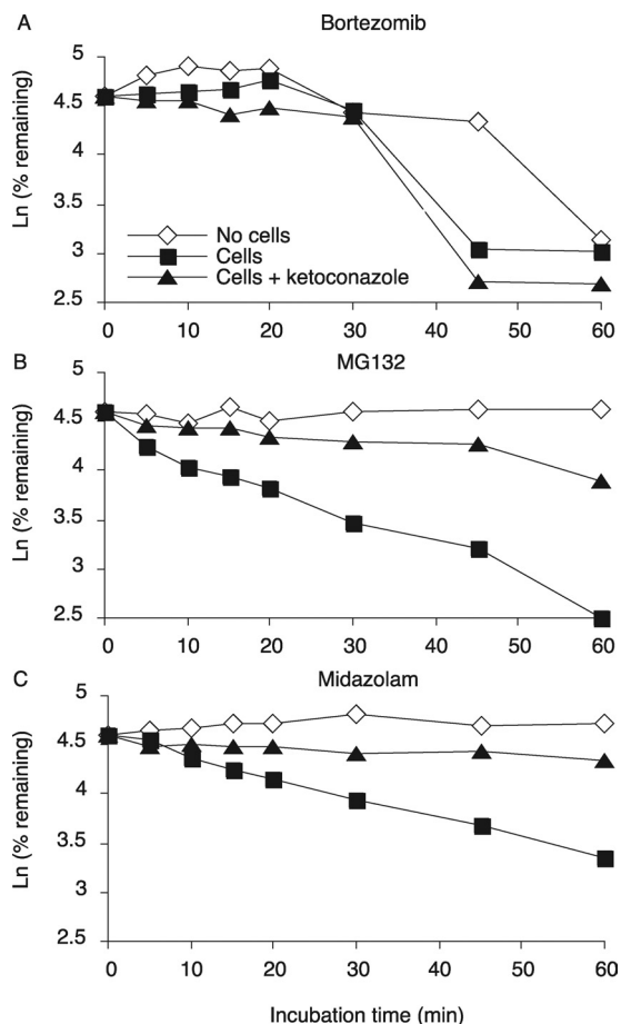
FIG. 7. Metabolic stability of proteasome inhibitors and midazolam using cryopreserved primary human hepatocyte cultures. The metabolism of bortezomib (A), MG132 (B), and midazolam (C) by cryopreserved primary human hepatocyte cultures was monitored by a substrate depletion method. Aliquots of the incubation media were taken at 0, 5, 10, 15, 20, 30, 45, and 60 min, and the quenched samples were analyzed by LC-MS/MS. Ketoconazole (1 \mu M) was used as a competitive inhibitor of CYP3A4.
