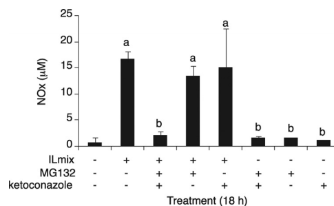
FIG. 4. Effect of ketoconazole on MG132 efficacy. Primary human hepatocytes (HH1410) were cultured for 3 days after delivery and treated with 1 mM PB for an additional 2 days. PB was maintained in the media during treatments. The cells were treated for 18 h with ILmix, ketoconazole (Ket, 10 \mu M), or MG132 (20 \mu M) in different combinations as indicated in the figure, and NO x was measured in the media. Values are the mean \pm S.D. of three independent samples. a, significantly different from control; b, significantly different from ILmix alone, P < 0.05 .
