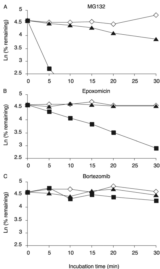
FIG. 6. Metabolic stability of proteasome inhibitors and midazolam using pooled human liver microsomes. The metabolism of MG-132 (A), epoxomicin (B), and bortezomib (C) by HLM were monitored by a substrate depletion method. Aliquots were taken from the incubation mixtures at 0, 5, 10, 15, 20, and 30 min, and the quenched samples were analyzed by LC-MS/MS. Ketoconazole (1 \mu M) was used as a competitive inhibitor of CYP3A4.
