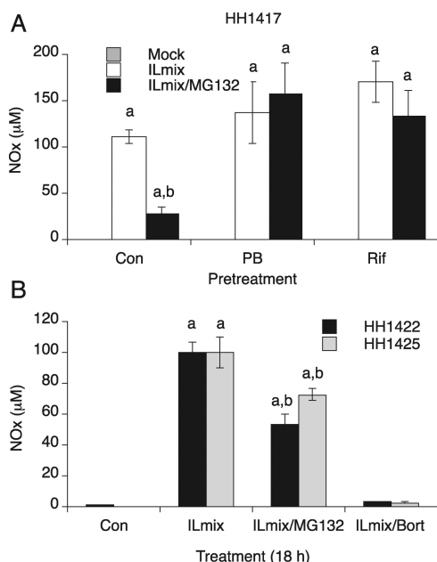
FIG. 3. Effect of pretreatment with PB and RIF on the efficacies of proteasome inhibitors. A, primary human hepatocytes (HH1417) were cultured for 3 days after delivery and treated with or without 1 mM PB or 50 \mu M rifampicin for an additional 2 days. PB or RIF were maintained in the media during treatments. Hepatocytes were treated with vehicle (mock), ILmix, or ILmix/MG132 (20 \mu M), and NO x was measured in the media 20 h after treatment. B, bortezomib efficacy on NO x production. Two different human hepatocyte preparations (HH1422 and HH1425) were pretreated with 1 mM PB for 2 days and then treated with vehicle ILmix, ILmix and MG132 (10 \mu M), or ILmix and bortezomib (Bort, 10 \mu M) for 18 h. NO x was measured in the media. Values are the mean \pm S.D. of three independent samples. a, significantly different from control; b, significantly different from ILmix alone, P < 0.05 . Con, control.
