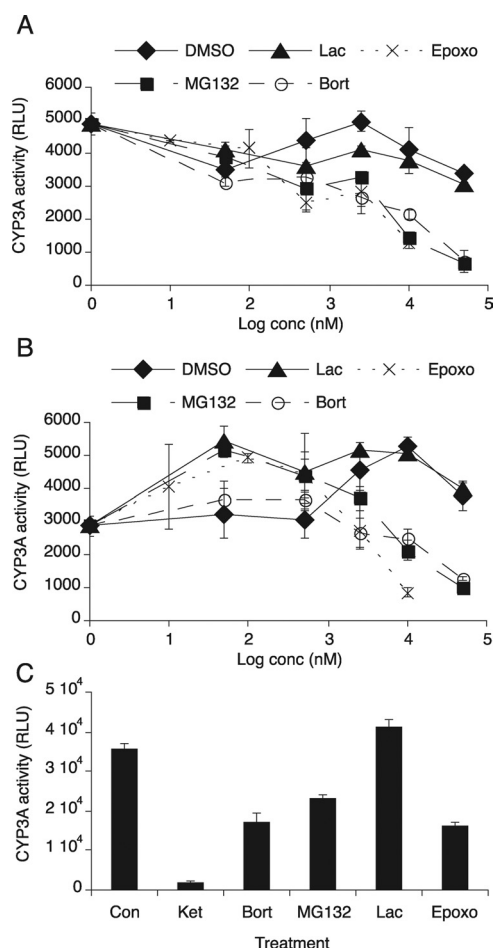
FIG. 5. Effect of proteasome inhibitors on CYP3A activity. CYP3A activity was measured by using the P450-Glo CYP3A4 assay system with Luciferin-PPXE as a substrate of CYP3A. A, CYP3A activity in pooled human liver microsomes. Luciferin-PPXE (100 \mu M) was mixed with either DMSO as a control or various concentrations (0.05–50 \mu M) of MG132, lactacystin (Lac), or bortezomib (Bort) or 0.01 \mu M to 10 \mu M epoxomicin (Epoxo) and then incubated with microsomes (1 \mu g/ml) for 10 min. The reaction was started by addition of NADPH. After 30 min, luminescence was measured with a luminometer. B, CYP3A4 activity in CYP3A4 Supersomes. Luciferin-PPXE was mixed with either DMSO as a control or various concentrations of proteasome inhibitors as described above and then incubated with CYP3A4 Supersomes (0.5 \mu g/ml) for 10 min. Thirty minutes after addition of NADPH to the reaction, luminescence was measured with a luminometer. C, hepatocellular CYP3A activity. Two-day PB-treated primary human hepatocytes (HH1425) were incubated with various proteasome inhibitors [20 \mu M MG132, 20 \mu M bortezomib, 10 \mu M clasto-lactacystin \beta -lactone (Lac), or 2.5 \mu M epoxomicin] or 20 \mu M ketoconazole (Ket) as a positive control (Con). Four hours later, hepatocytes were incubated with 25 \mu M Luciferin-PPXE for 1 h, and the media were collected for luminescence assay as described above. Values are the mean \pm S.D. of three independent samples. RLU, relative light units.
