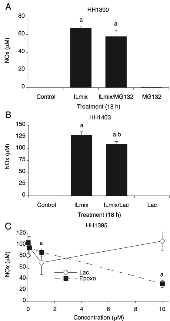
Fig. 2. NO _x production of primary human hepatocytes and its inhibition by proteasome inhibitors. Primary human hepatocytes were cultured for 3 days after delivery and treated with 1 mM PB for an additional 2 days. PB was maintained in the media during treatments. NO _x was measured from media after treatment. A, hepatocytes (HH1390) were treated with ILmix ( 2.5 ng/ml IL- 1\beta , 5 ng/ml TNF- \alpha , and 5 ng/ml IFN- \gamma ), the proteasome inhibitor MG132 ( 10 \mu\text{M} ), or both for 18 h. B, hepatocytes (HH1403) were treated with ILmix, the proteasome inhibitor lactacystin ( 10 \mu\text{M} ), or both or ILmix/lactacystin ( 10 \mu\text{M} ) for 18 h. C, concentration dependence of the effects of proteasome inhibitors on NO _x production. PB-treated hepatocytes (HH1395) were cotreated with ILmix and various concentrations of lactacystin (Lac) or epoxomicin (Epoxo) for 18 h, and NO _x was measured in the media. Values are the mean \pm S.D. of three independent samples. a, significantly different from control; b, significantly different from ILmix alone, P < 0.05 .
