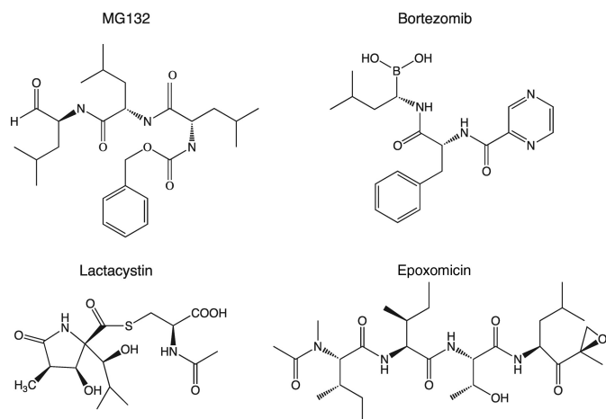
Fig. 1. Structures of the proteasome inhibitors used in this study.
