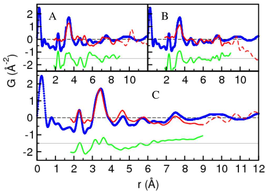
Figure 6. PDF crystal model fits of TMPC precursor. A) Fit from crystallized 12-member ring structure of LeBlanc and Lock 16 . B) Fit from crystallized cluster model of Heaven et al. 22 C) Fit from double-helix structure of Bau 23 . The blue circles are the 80 K PDF data, the solid red line is the calculated PDF of the best-fitting model over the range of r from 1.8 – 9 Å, and the dashed red line is the PDF from the refined model extended out to 12 Å. The green line is the difference between the data and fit over the fit range and is offset for clarity.
