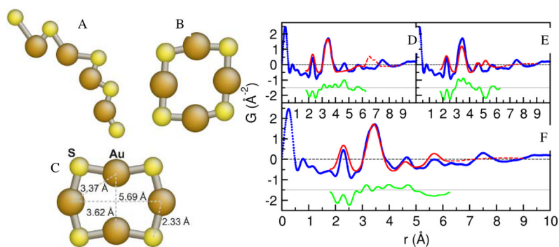
Figure 5. PDF molecular models of TMPC precursor. A) Refined 9-member straight-chain polymer model. B) Refined 8-member closed-chain model. C) Refined 8-member ring model. Model bond length values are shown. D, E, F) PDF fits corresponding to A, B, C, respectively. In the PDF fits the blue circles are the 80 K data, the solid red line is the calculated PDF of the best-fitting model over the range of r from 1.8 – 6.25 Å, and the dashed red line is the PDF from the refined model extended out to 9 Å. The green line is the difference between the data and fit over the fit range and is offset for clarity.
