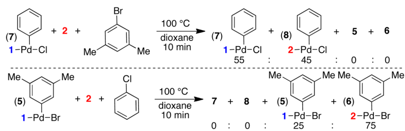
Figure 5. Competition experiment to distinguish between pathway 1 and pathway 2.
