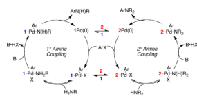
Figure 6. Proposed mechanism of the mixed-ligand catalyst system.
