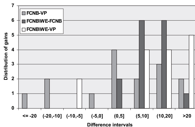
Figure 1 Histogram summarizing the work saved over sampling results for factorized complement naïve Bayes (FCNB)/weight engineering (WE), FCNB and voting perceptron (VP). The x-axis shows the discretized differences between the methods (FCNB - VP, FCNB/WE - FCNB, FCNB/WE - VP), and the y-axis shows for how many topics (drug reviews) the given difference in performance occurs. Looking at the white bars, we observe that most of the topics are to the right of 0 on the x-axis, visualizing the advantage of FCNB over VP. Looking at the light grey bars, we observe that, except for two reviews, they are to the right of 0, meaning that FCNB/WE performs better than VP on 13 out of 15 drug groups. Looking at the dark grey bars, we observe that all the bars are in the right half of the interval, visualizing the clear advantage of weight management when using FCNB.
