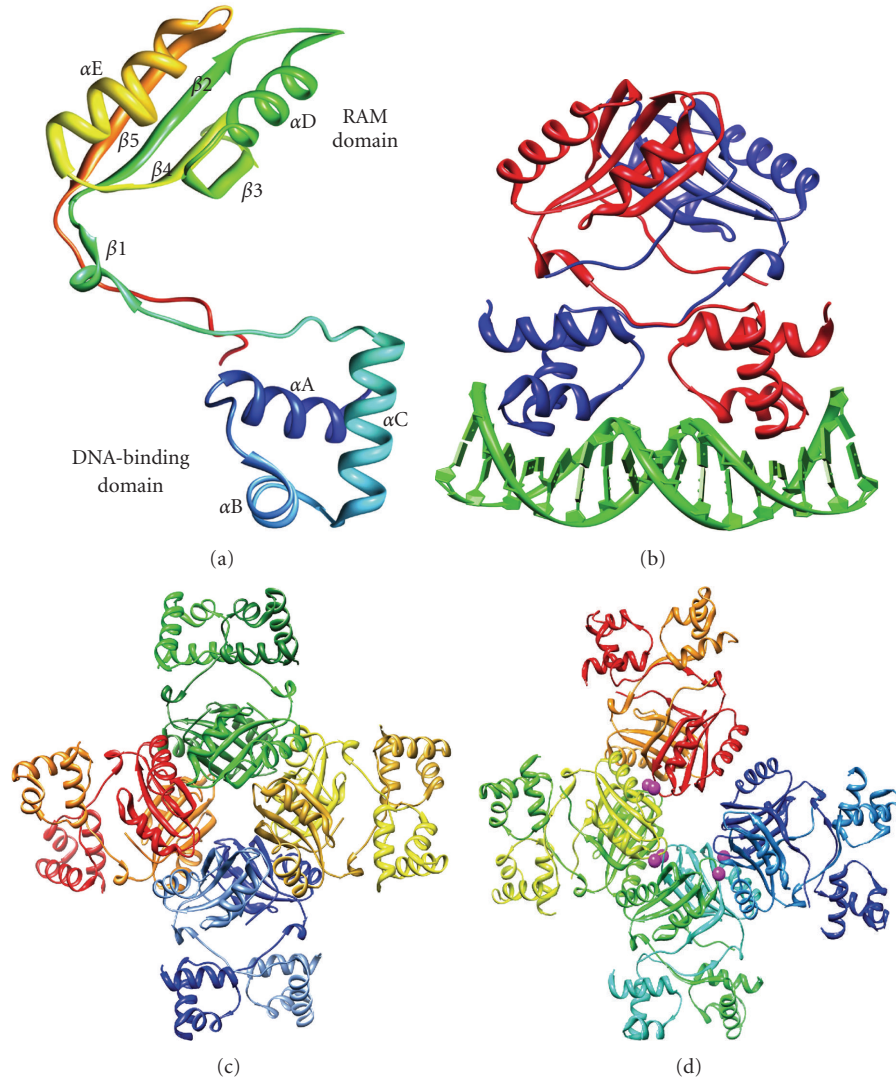
FIGURE 1: Structural features of archaeal Lrp-like proteins. (a) Monomeric structure of Grp from S. tokodaii (PDB 2E7W) [31]. Secondary structure elements are named as follows: \alpha -helices are called \alpha A – \alpha E and \beta -strands \beta 1 – \beta 5 . The N-terminal DNA-binding domain corresponds to the bottom part of the structure, the C-terminal ligand binding domain to the top part. These are labeled DNA-binding domain and RAM domain, respectively. (b) Cocystal structure of an FL11 dimer bound to DNA (PDB 2E1C) [30]. (c) Octameric structure of LrpA from P. furiosus (PDB 1I1G) [28]. (d) Cocystal structure of an arginine-bound octamer of FL11 from P. horikoshii , which has an open conformation (PDB 2ZNY) [32]. The position of the arginine molecules is shown by purple symbols.
