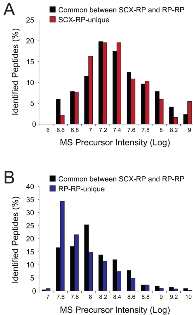
Figure 4. Histogram plots of MS precursor intensities for peptides detected by both fractionation techniques ( black bars ) and for those peptides identified uniquely by SCX-RP ( A, red bars ) and RP-RP ( B, blue bars ), respectively.
