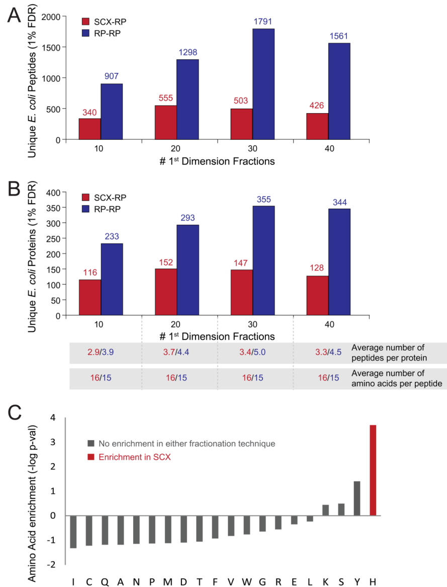
Figure 2. Analysis of tryptic peptides derived from e.coli lysate by SCX-RP ( red ) and RP-RP ( blue ) fractionation. RP-RP provided for higher numbers of identified ( A ) peptides and ( B ) proteins as compared to SCX-RP for independent experiments spanning 10, 20, 30, and 40 first dimension fractions, respectively. The number of peptides identified per protein was slightly higher for RP-RP, while peptide length was on average shorter by one amino acid ( B, bottom ). A permutation test ( C ), revealed that peptides identified by SCX-RP exhibited a statistical bias for histidine ( -\log[p\text{-val}] > 2 ) residues as compared to those identified by RP-RP.
