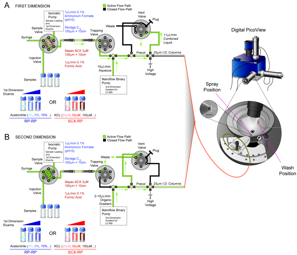
Figure 1. Schematic diagram of automated, online nanoflow RP-RP platform. (A) The autosampler loads peptides and then is used to inject salt or organic eluents to generate first dimension SCX (red) or RP (blue) fractions, respectively. First dimension fractions are diluted (10 \times ) and acidified with reversed phase A solvent (0.1% formic acid, 3% acetonitrile) introduced by an ultra-high pressure binary pump. An additional 6-port, 2-position valve provides a vented second dimension column configuration, and ensures efficient capture of peptides onto the precolumn. (B) The ultra-high pressure binary pump delivers an organic gradient to elute peptides from the second dimension column for MS/MS analysis. The vent valve generates an effluent split of \approx 1000:1 to provide a stable column/ESI flow rate of \approx 5 nL/min. Active solvent flow paths are highlighted in green. (right) A computer-controlled positioning platform (Digital PicoView) automatically moves the emitter tip beneath a wash station for sample loading in-between fractions.
