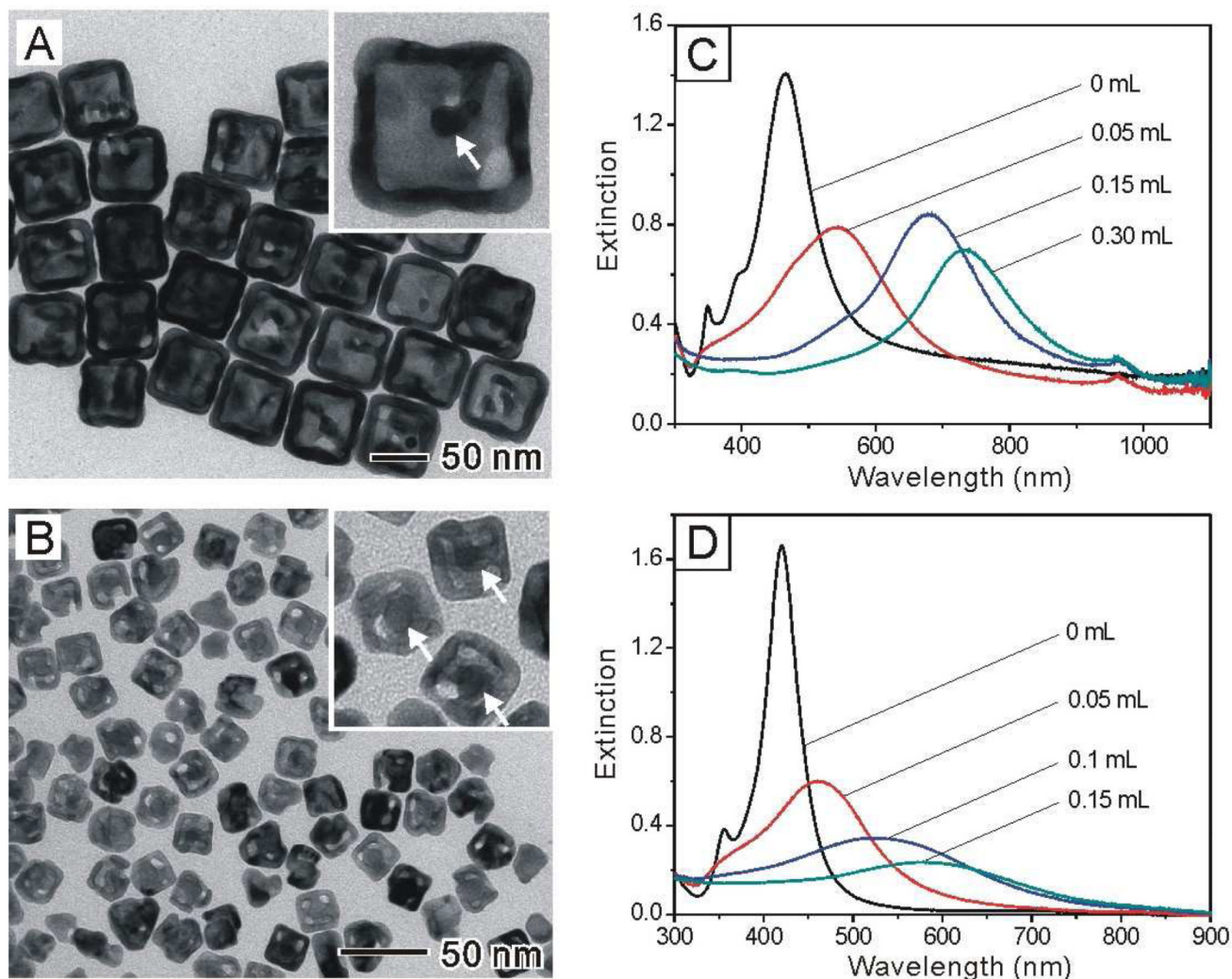
Figure 8. TEM images of Au-based nanocages derived from the Au@Ag nanocubes of (A) 50 nm and (B) 21 nm in edge length, respectively. The wall thicknesses of the Au nanocages were (A) 8.8 \pm 0.9 nm, and (B) 4.2 \pm 0.4 nm, respectively. Insets show the corresponding images at higher magnification, clearly revealing the existence of the original Au seeds in the interiors (marked by white arrows). (C, D) UV-vis extinction spectra taken from aqueous suspensions of Ag nanocubes (C) 50 nm and (D) 21 nm, respectively, in edge length after they had been titrated with different volumes of an aqueous 0.5 mM HAuCl 4 solution (as labeled on each curve).
