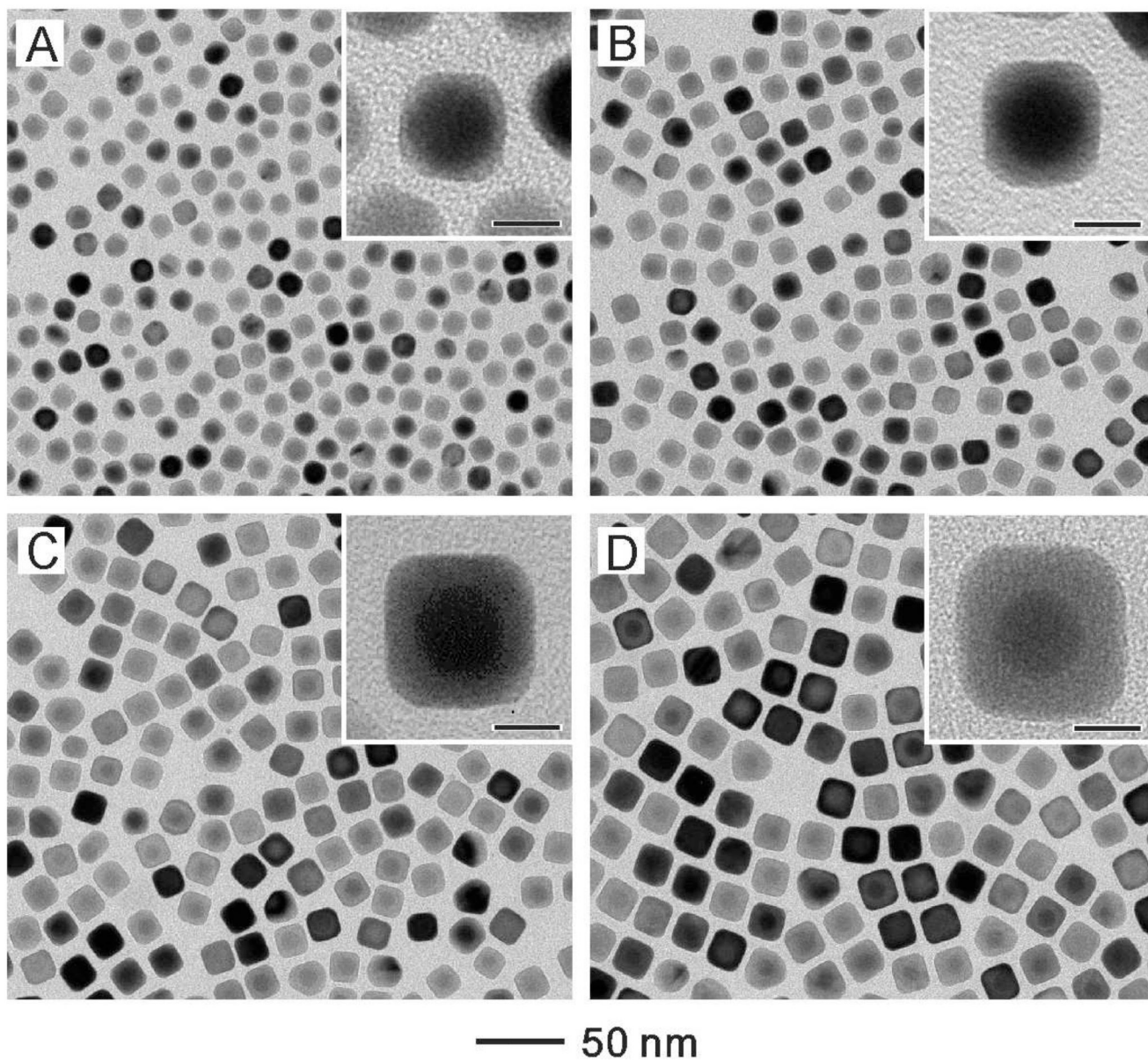
Figure 2. TEM images of Au@Ag core-shell nanocubes obtained by injecting different volumes of AgNO 3 (2 mM) into 5 mL solutions containing the same amount of Au seeds (14.6 mg/L) at 60 °C. The volumes of AgNO 3 were: (A) 0.25 mL (edge length of the cubes: 13.4±0.6 nm), (B) 0.5 mL (edge length of the cubes: 15.2±0.6 nm), (C) 1 mL (edge length of the cubes: 17.2±0.7 nm), and (D) 2 mL (edge length of the cubes: 20.0±0.6 nm). After injection, the final concentrations of AgNO 3 were 0.09, 0.17, 0.29, and 0.44 mM, respectively. Insets are the corresponding high-magnification TEM images with the scale bars being 8 nm.
