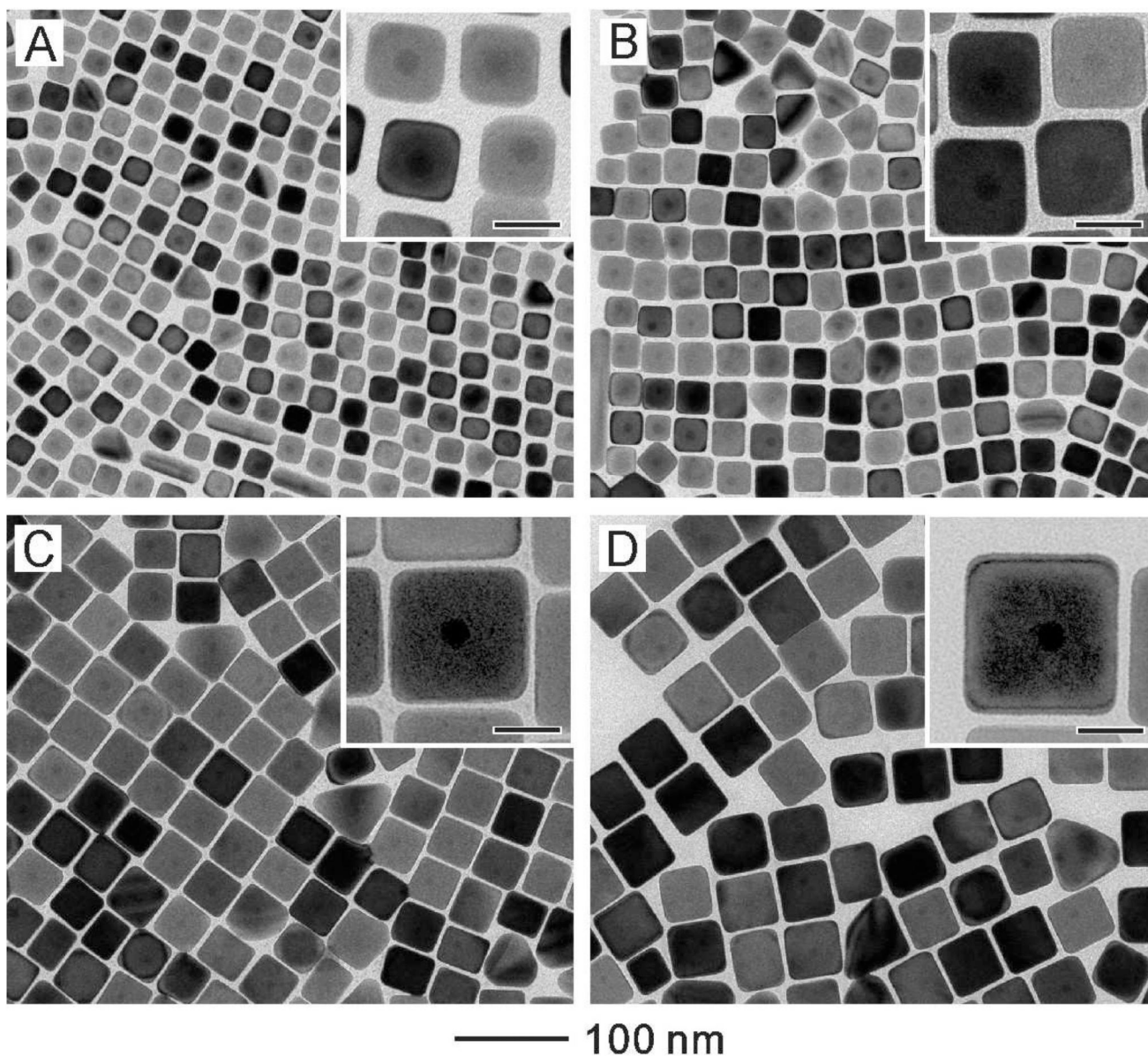
Figure 3. TEM images of Au@Ag core-shell nanocubes obtained by injecting 5 mL AgNO 3 solution (2 mM) and 5 mL AA solution (50 mM) into 5 mL of solutions with different seed concentrations: (A) 14.6 mg/L (edge length of the cubes: 24.4 \pm 0.9 nm), (B) 7.3 mg/L (edge length of the cubes: 30.4 \pm 1.2 nm), (C) 2.9 mg/L (edge length of the cubes: 42.6 \pm 1.7 nm), (D) 1.46 mg/L (edge length of the cubes: 50.4 \pm 2.2 nm). After injection, the final concentration of AgNO 3 was 0.67 mM. The reaction temperature was controlled at 60 °C. Insets are the corresponding high-magnification TEM images with the scale bars being 20 nm.
