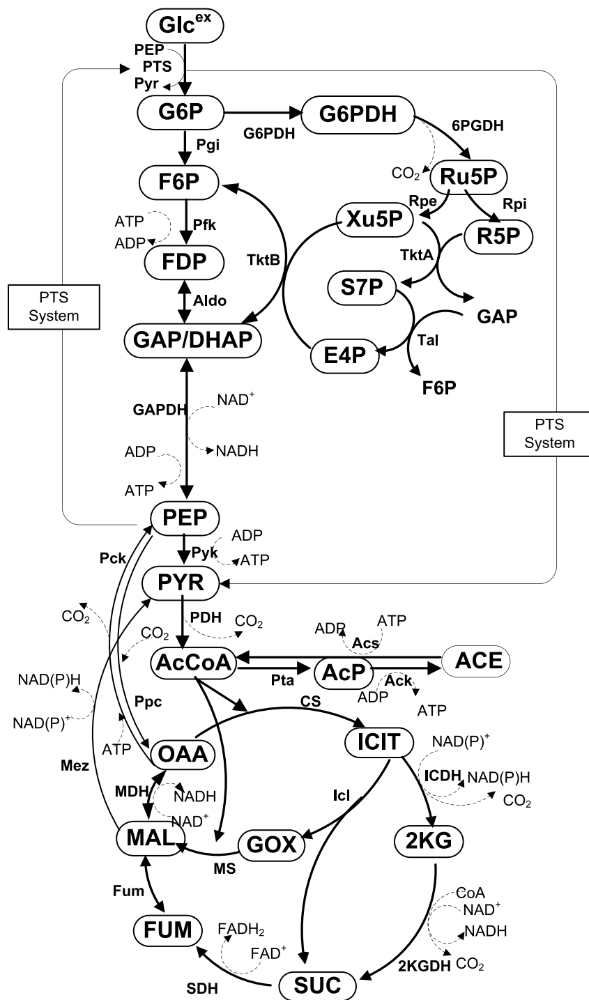
Figure 1 Metabolic pathways considered in this simulation.
