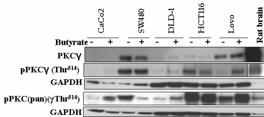
Fig. 4. The expression levels of PKC \gamma , pPKC \gamma -Thr 514 and pPKC(pan)( \gamma Thr 514 ) in Caco2, SW480, DLD-1, HCT116 and Lovo cells. Comparison with authentic PKC \gamma from rat brain. Cells were treated with 10 mM butyrate for 24 h. Lysates were subjected to Western blot analysis with antibodies as described in Materials and methods . GAPDH was probed as a loading control. Representative blots are shown.
