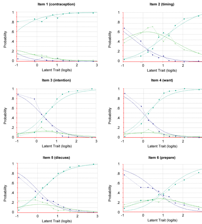
Figure 3. Item Characteristic Curves a for LMUP items Notes: a The x-axes represent total LMUP score. The y-axes represent probability of selecting a given response. Each of the three smoothed lines represents the probability that respondents with a given LMUP score selected each of three available responses. For instance, on item 5 (discuss), the lowest response category (never discussed having children) was the most common response among participants with the lowest LMUP scores. The highest response category (agreed to become pregnant) was the most common among participants at all LMUP levels above 0 logits.
