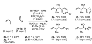
Scheme 3. Iridium catalyzed reductive coupling of butadiene to aldehydes 2e-2g and 2i .
