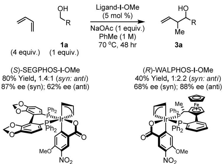
Scheme 4. Preliminary evaluation of chirally modified catalysts.
