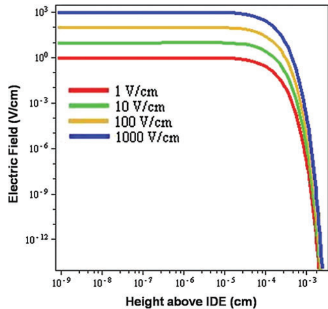
FIG. 3. Graphical depiction of electric field at different magnitudes above the interdigitated electrode plane demonstrating its exponential decay with height. Color images available online at www.liebertonline.com/ten .
