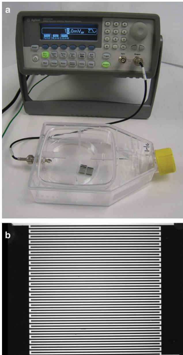
FIG. 2. Image of interdigitated electrode assembled in flask (a) and close-up image of interdigitated electrode showing contact pads and electrode array (b). The bright (white) regions are glass, whereas the dark regions are metal. Color images available online at www.liebertonline.com/ten .
