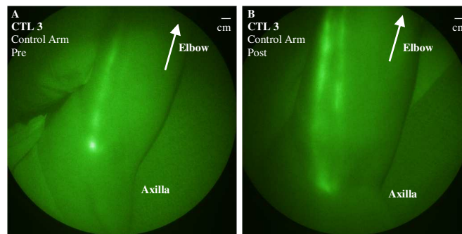
Fig. 4. The upper arm and axilla of Control Subject 3 before PCD treatment (A, Media 1) and after PCD treatment (B, Media 2). After treatment, recruitment of vessels and increased rate of propulsion are observed.
