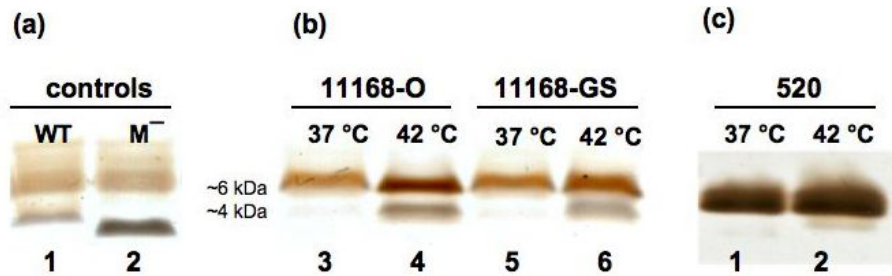
Figure 1 Silver-stained SDS-PAGE gel of the LOS extracted from C. jejuni NCTC 11168 and 520. (a) Controls of M. catarrhalis serotype A (strain 2951) LOS for relative sizing LOS. Lanes: 1, M. catarrhalis wild-type LOS (WT); 2, M. catarrhalis M - mutant LOS lacking the terminal glucose; (b) C. jejuni 11168-O and 11168-GS LOS extracted from bacteria grown at 37°C and 42°C. Lanes: 3, 11168-O at 37°C; 4, 11168-O at 42°C; 5, 11168-GS at 37°C; 6, 11168-GS at 42°C. (c) C. jejuni 520 LOS extracts from bacteria grown at 37°C and 42°C. Lanes: 1, 520 at 37°C; 2, 520 at 42°C. Higher-M r LOS resolved at ~6 kDa and lower-M r LOS at ~4 kDa.
