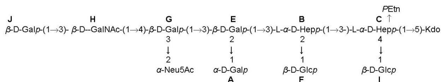
Figure 2 C. jejuni NCTC 11168 core OS structure. Shown is the structure of the higher-M r LOS form [20,21], the lower-M r form can lack the Neu5Ac residue thereby producing an asialo-GM 1 mimic. Abbreviations: Gal, galactose; GalNAc, N-acetylgalactosamine; Glc, glucose; Hep, heptose; Neu5Ac, N-acetylneuraminic acid; Kdo, 3-deoxy-D-manno-oct-2-ulosonic acid; PEtn, phosphorylethanolamine.
