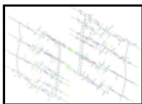
Fig. 3. Crystal packing of title compound viewed along the c axis. The \pi - \pi interactions are shown as black dashed lines.
