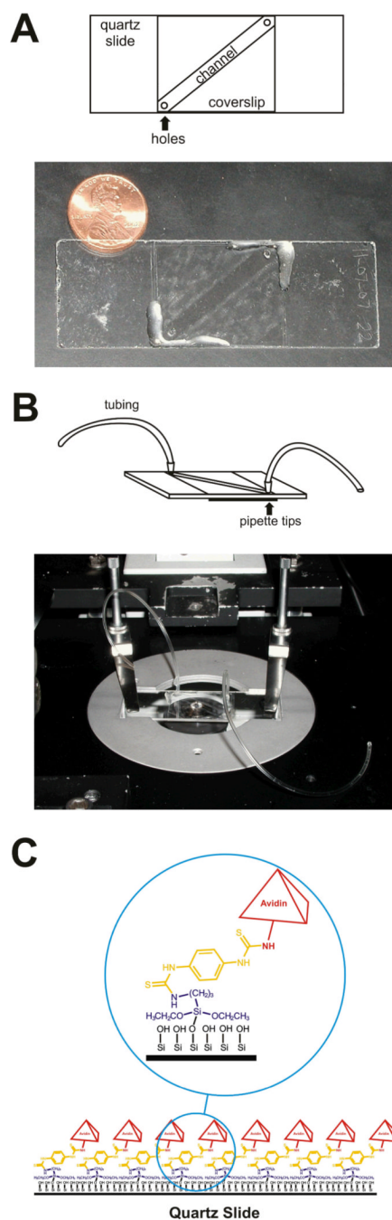
Figure 2. Microscope slide preparation. (A) A fluidic channel is created between the two 1-mm holes in the quartz slide by sandwiching two pieces of double-sided sticky tape between the slide and the coverslip. (B) Tubing for fluid introduction and disposal is attached to the holes in microscope slide by using pipette tips. Epoxy resin is added to generate a tight seal between the tubing and pipette tips as well as between the pipette tips and holes. Note that, when placed on the microscope stage, the coverslip is face-down, allowing the tubing on the microscope slide to be face-up. (C) The slide is densely coated with avidin (red) covalently bound via a PDTIC linker (yellow) to an aminosilanzed (blue) quartz slide (black) surface.
