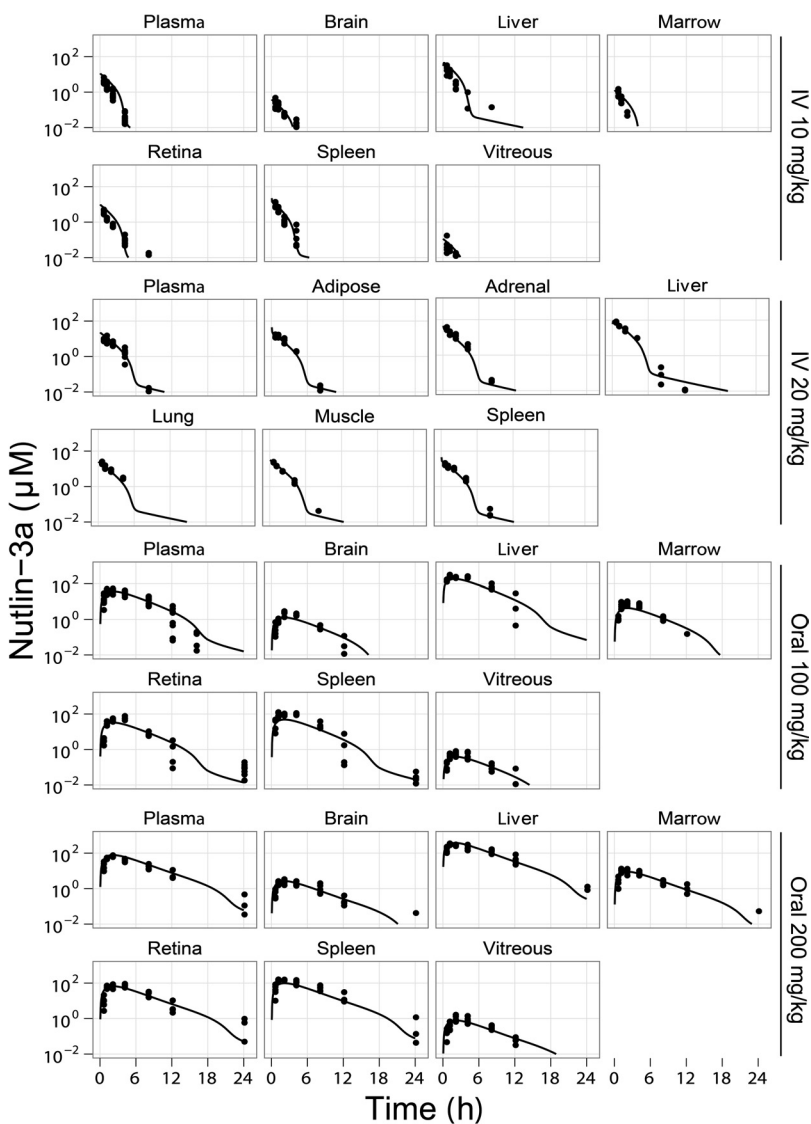
FIG. 3. Concentration-time plots of nutlin-3a in tissues. Symbols are data points from individual mice, and the lines represent the model-predicted concentrations. Data from the 50 mg/kg oral group are not shown. Data below the lower limit of quantitation are not shown.
