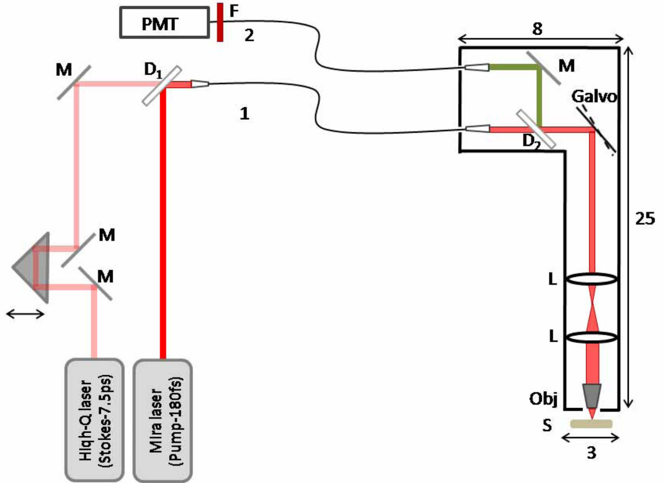
Fig. 1. Schematic diagram of the fiber-delivered probe for CARS tissue imaging: M-mirrors; D1- 1000 nm longpass dichroic mirror; D2- 760 nm longpass dichroic mirror, L-lens; Obj-objective; S-sample; F- 670 nm bandpass filter. Fiber 1 is used for delivery of the excitation pulses and fiber 2 is used for detecting the CARS radiation. The dimensions of the probe are indicated in cm.
