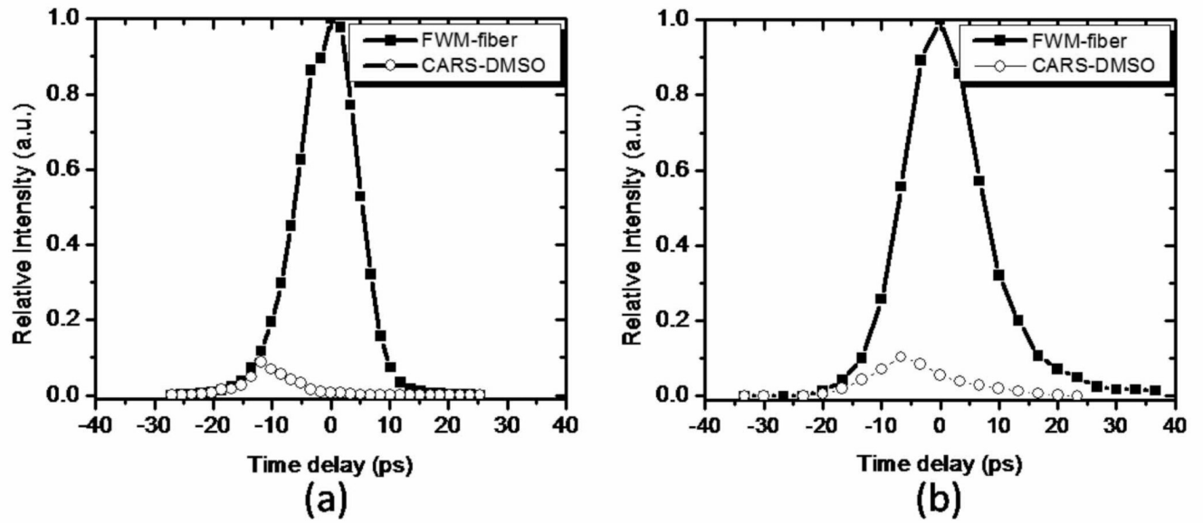
Fig. 4. CARS signal intensity from the DMSO sample and FWM from the fiber as a function of time delay between the pump and the Stokes beam for the DCPCF16 fiber (a) and the LMA-20 fiber (b).
