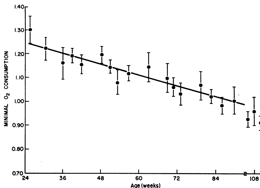
FIGURE 2 Decline in MOC between 24 and 108 wk of age in the female rat. MOC values are given for 8-20 female rats per point of the same strain as in Fig. 1. Standard deviations are indicated by vertical bars. All rats were fed a low iodine diet.
