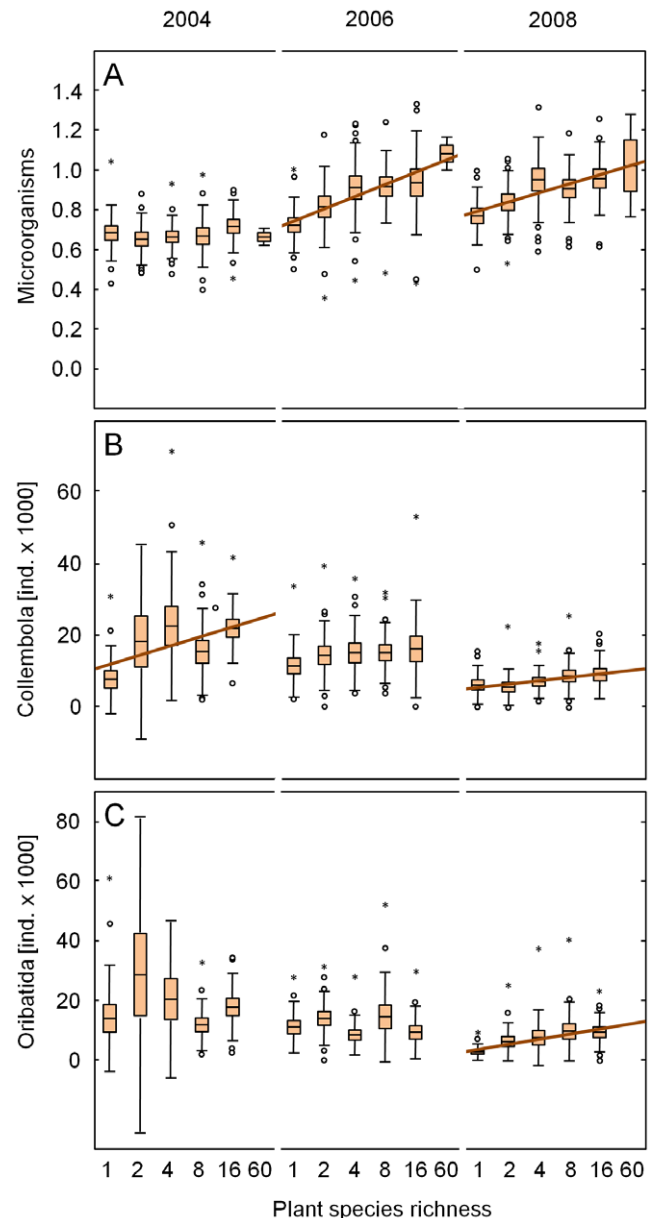
Figure 1. Plant species richness effects on soil microorganisms and mesofauna. Variations in (A) soil microbial biomass [ \text{mg C}_{\text{mic}} \text{g}^{-1} soil dry weight], and the density of (B) Collembola, and (C) Oribatida [all individuals \text{m}^{-2} ] as affected by plant species richness in different years. Regression lines indicate significant effects ( P < 0.05 ); brown lines indicate decomposers in the broader sense (including microbivores); means (lines) with standard error (boxes), standard deviation (error bars), extremes (dots) and outliers (asterisks). doi:10.1371/journal.pone.0016055.g001
