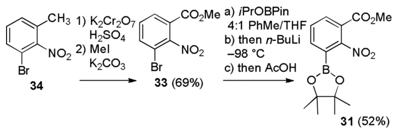
SCHEME 8. Synthesis of Pinacol Boronate 31
