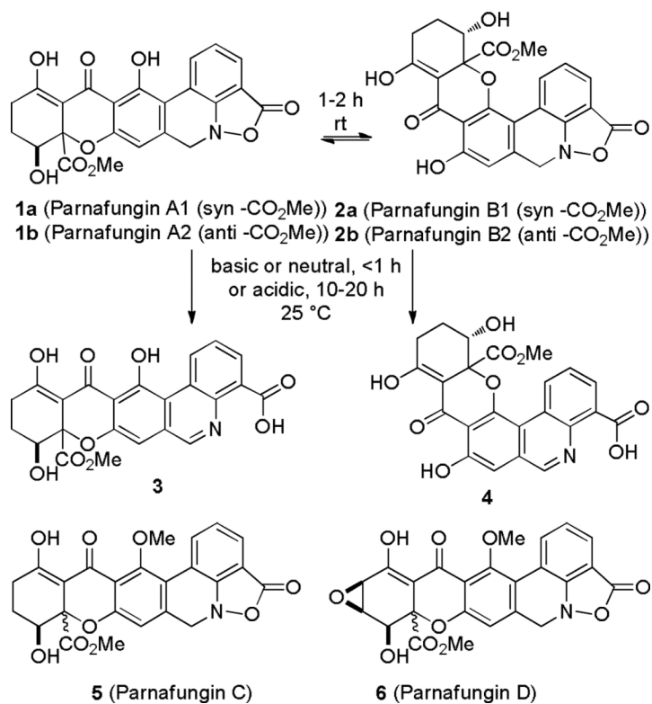
SCHEME 1. Parnafungin Structures and Decomposition Products
