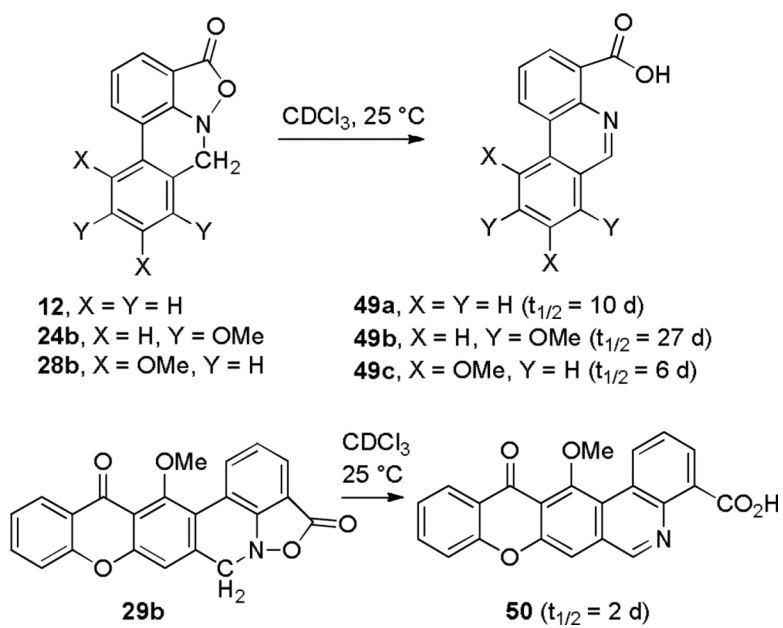
SCHEME 12. Decomposition of Benzisoxazolinones 12 , 24b , 28b and 29b
