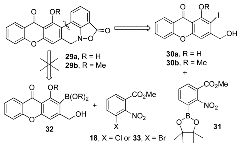
SCHEME 7. Retrosynthesis of Hexacyclic Models 29a and 29b
