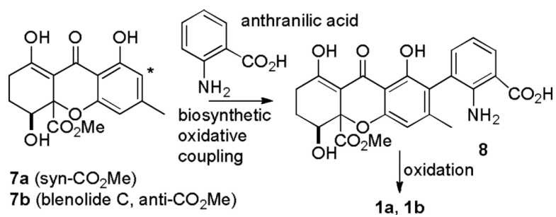
SCHEME 2. Possible Biosynthesis of the Parnafungins
