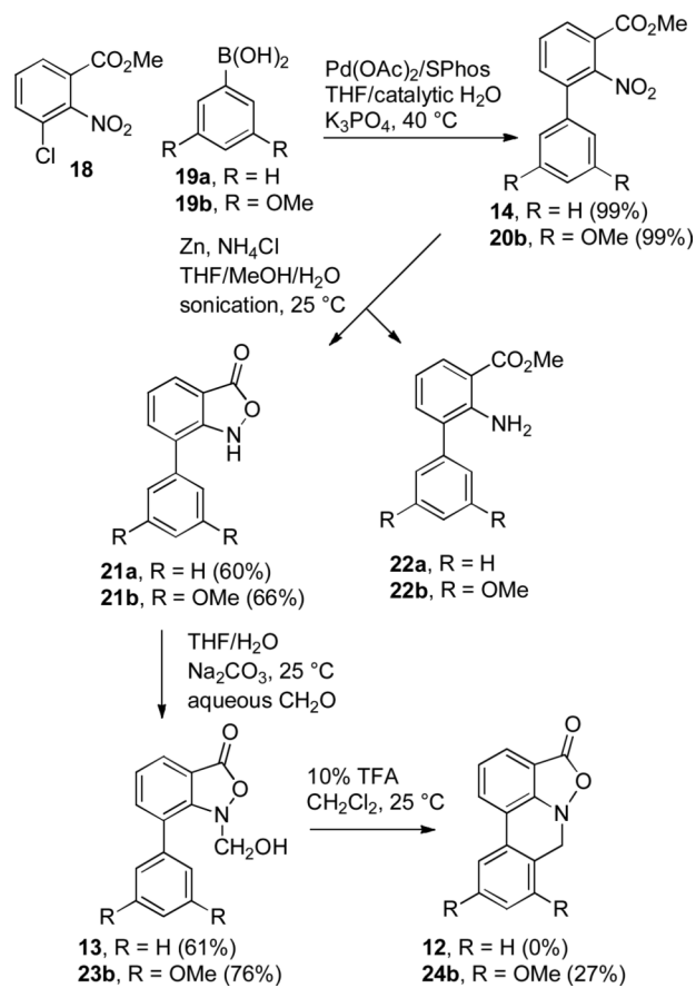
SCHEME 5. Synthesis of Tetracycle 24b
