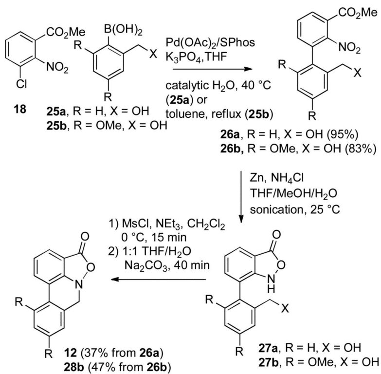
SCHEME 6. Synthesis of Tetracycles 12 and 28c
