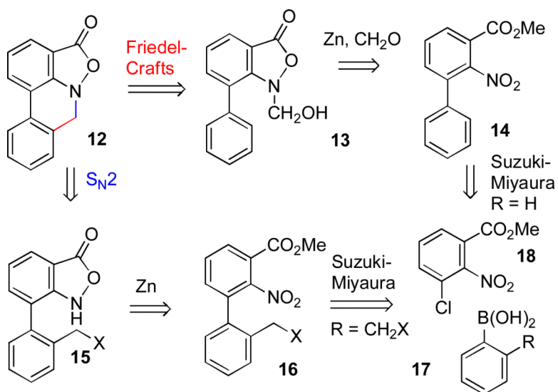
SCHEME 4. Retrosynthesis of Tetracycle 12
