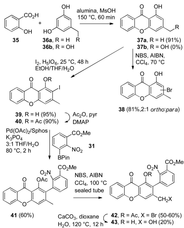
SCHEME 9. Unsuccessful Route to 43
