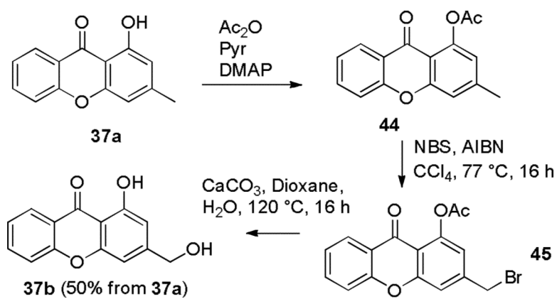
SCHEME 10. Oxidation of 37a to give 37b
