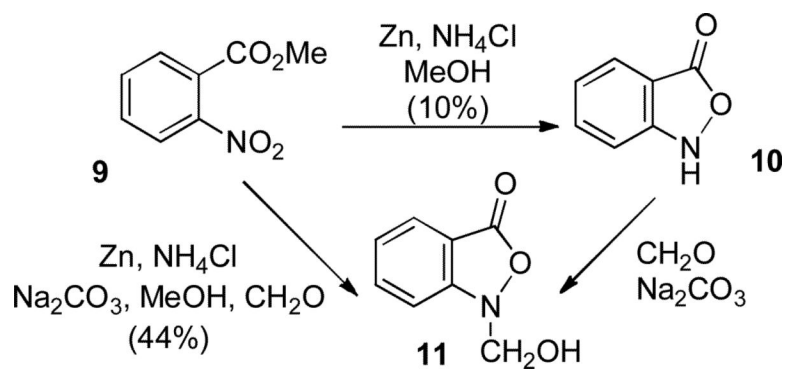
SCHEME 3. Wierenga Benzisoxazolinone Synthesis
