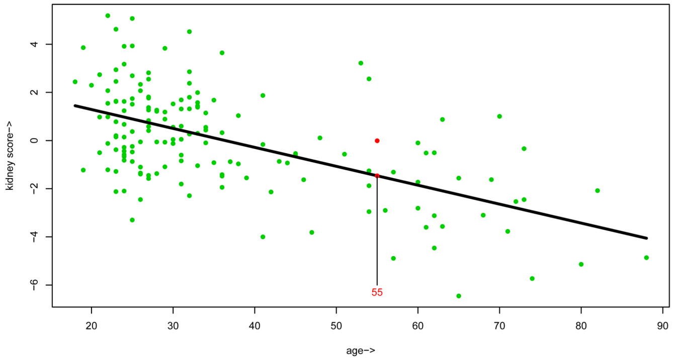
Figure 2. Kidney function plotted versus age for 157 healthy volunteers from the nephrology laboratory of Dr. Brian Myers. The least squares regression line has a strong downward slope. A new donor age 55 has appeared, and we need to predict his kidney score.
