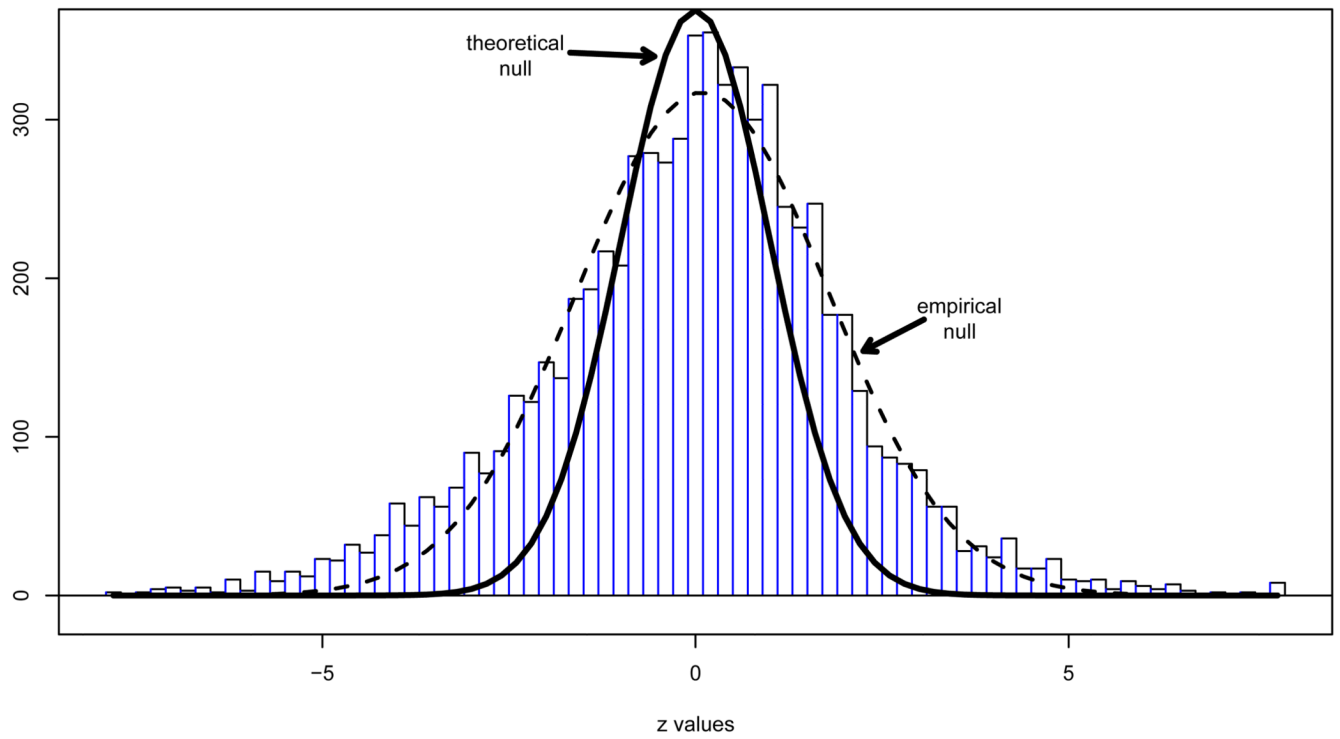
Figure 5. Histogram of z -values for N = 7128 genes in a microarray study comparing two types of leukemia. The N(0, 1) theoretical null is much narrower than the histogram center; a normal fit to the central histogram height gives empirical null N(.09, 1.68^2) . Both curves have been scaled by their respective estimates of p_0 in (7).
