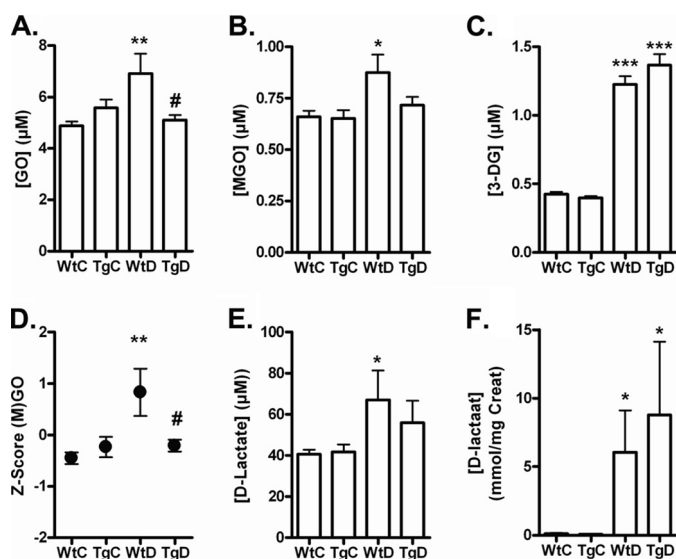
FIGURE 2. Oxo-aldehyde formation and detoxification of (M)GO in the blood of wild-type and transgenic GLO-1 rats. Glyoxal (A), MGO (B), and 3-DG (C) levels in the blood of WtC, TgC, WtD, and TgD rats are shown. A composite score was calculated for the GLO-1-sensitive oxo-aldehydes GO and MGO (D). D-Lactate levels in the plasma (E) and urine (F) of the WtC, TgC, WtD, and TgD rats are shown. * p < 0.05 compared with control; ** p < 0.01 compared with control; *** p < 0.001 compared with control; # p < 0.05 compared with wild-type diabetic.
