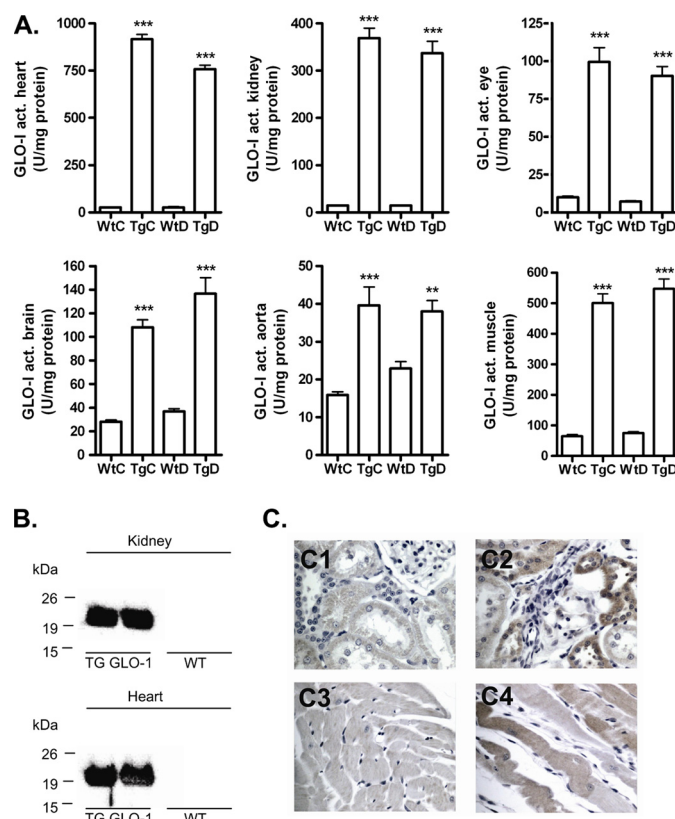
FIGURE 1. GLO-1 activity and human protein expression in tissue of wild-type and transgenic GLO-1 rats. A, shown is GLO-1 enzyme activity ( act. ) in lysates of heart, kidney, eye, brain, aorta, and gastrocnemius muscle tissue of WtC, TgC, WtD, and TgD rats. B, shown is a Western blot of human GLO-1 protein overexpression in transgenic heart and kidney compared with wild-type heart and kidney lysates. C, immunohistochemistry of GLO-1 protein overexpression in transgenic heart (C2) and kidney (C4) compared with wild-type (C1, C3) is shown. ** p < 0.01 compared with control; *** p < 0.001 compared with control.
