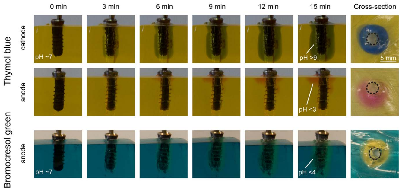
Figure 3. Proof of pH changes during electrochemical implant treatment. Photographic images of dental implants in simulated soft tissue using pH-sensitive dyes to visualize local pH changes. The dark blue color for thymol blue indicated a pH above 9 (alkaline) while the pink color confirmed a pH below 3 (strongly acidic). Confirmation with a second pH-sensitive dye, bromocresol green allowed mapping a similar acidic pH at the anode. For both dyes, a homogenous, circular simulated soft tissue section of high/low pH evolved around the implant insertion hole. doi:10.1371/journal.pone.0016157.g003
