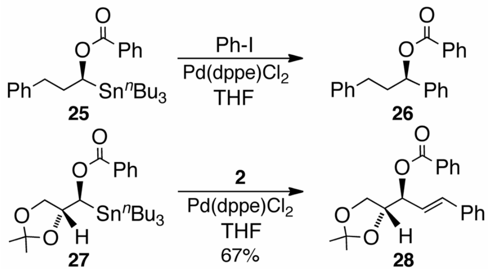
Figure 1. Cross-Coupling of Enantioenriched Stannanes
