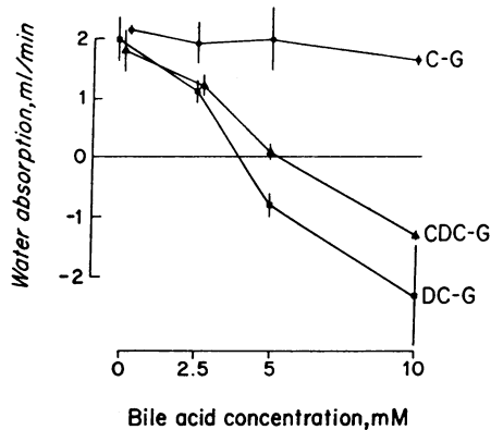
FIGURE 1 Fluid absorption from 25 cm segment of human jejunum (mean \pm SE; N=3 or 4 ) perfused with isotonic electrolyte solution and with conjugated trihydroxy (C-G) or dihydroxy (DC-G, CDC-G) bile acid solutions. Negative values represent fluid secretion.
