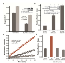
Figure 3. Reducing off-target phosphorylation of MEF2A-CSox in unfractionated cell lysates. a) Reactions were conducted using 1 \mu M substrate and 10 \mu g of the indicated HeLa lysate with or without the addition of staurosporine. The inset shows a western blot analysis of the indicated lysates, demonstrating p38 activation upon stimulation. b) The relative reaction slopes obtained using 1 \mu M substrate and 5 \mu g of the indicated lysates are shown. The inset shows a western blot analysis of each lysate. c) Initial phosphorylation reactions using 10 \mu g of total cellular protein from the indicated HeLa cell lysate demonstrated that MEF2A-CSox (1 \mu M) could report on the presence of active p38. Data is corrected for lag times, see Methods. d) Assays were performed using lysates from serum-starved or stimulated cells (10 \mu g) with MEF2A-CSox (1 \mu M). Inhibitors of p38 \alpha were added to the reactions containing lysates from stimulated cells where indicated. All reactions contained 1 \mu M staurosporine unless otherwise noted.
