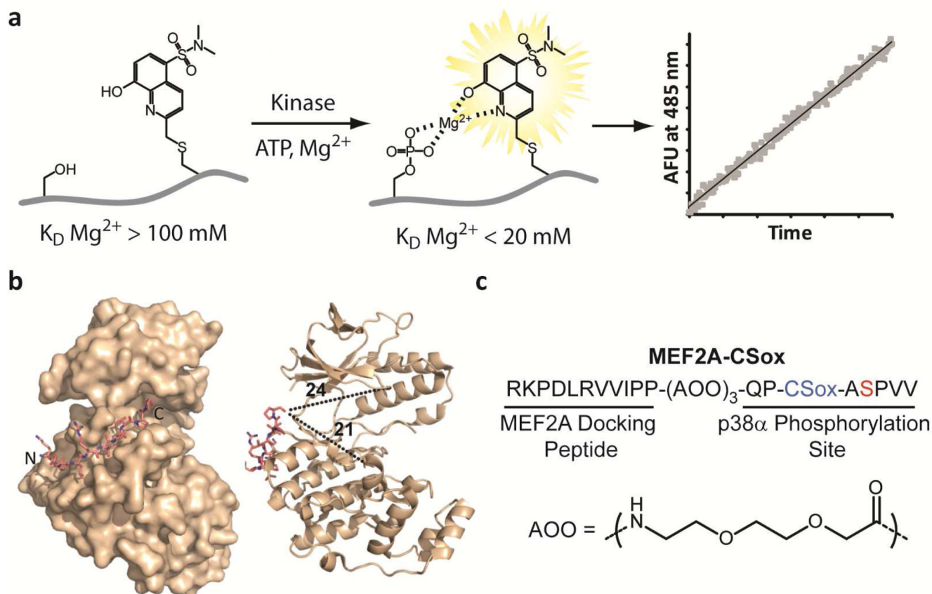
Figure 1. Rational design of a p38 \alpha chemosensor. a) A schematic of the chelation-enhanced fluorescence of the CSox amino acid upon phosphorylation. b) A crystal structure of the MEF2A docking peptide bound to p38 \alpha (left) and distances in Å from the C-terminus of the docking peptide to representative distal regions of the catalytic and substrate-binding domains of the kinase are shown (right) (18). c) The amino acid sequence of the MEF2A-CSox sensor with the position of CSox (blue) and the site of phosphorylation (red) indicated. The flexible 8-amino-3,6-dioxaoctanoic acid (AOO) linker is also shown.
