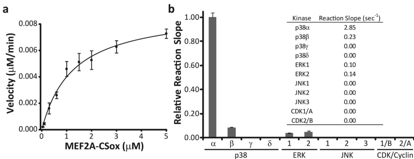
Figure 2. MEF2A-CSox is a substrate for recombinant p38 \alpha . a) A direct fit of a velocity versus MEF2A-CSox concentration plot using the Briggs-Haldane equation. b) Phosphorylation reactions were conducted with the indicated recombinant kinase (15 nM) using 1 \mu\text{M} substrate and demonstrate that MEF2A-CSox is selective for p38 \alpha among these kinases. The inset shows the average reaction slope for each kinase.
