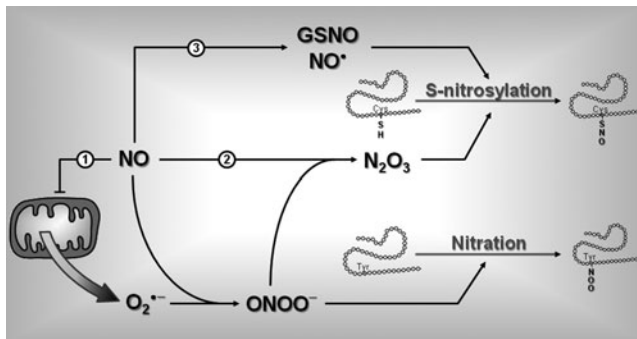
FIG. 7. Role of NO in protein posttranslational modification. Increased NO production can alter protein structure and ultimately function by nitration ((1)) and/or S-nitrosylation ((2), (3)). (1) NO can inhibit mitochondrial cytochrome c and stimulate generation of anion superoxide ( O_2^{\bullet-} ). Interaction between NO and O_2^{\bullet-} forms peroxynitrite ( ONOO^- ). ONOO^- can react with a free Tyr on proteins to form nitrated Tyr through a reaction called tyrosine nitration. (2) ONOO^- can also react with another molecule of NO to form dinitrogen trioxide ( N_2O_3 ). N_2O_3 can interact with free Cys thiols on proteins to form S-nitro-thiol groups in a reaction called S-nitrosylation. (3) In an oxidative environment, increased NO level can also increase formation of GSNO and/or reactive NO ( NO^* ). GSNO and NO^* can also interact with free Cys to induce S-nitrosylation. Cys, cysteine; GSNO, nitroso-glutathione; Tyr, tyrosine.
