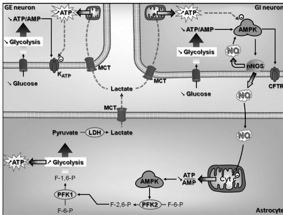
FIG. 6. Hypothetical role of NO production by VMN GI neurons in the astrocyte-neuron lactate shuttle. Decreased extracellular glucose decreases GI neuronal intracellular ATP/AMP ratio and increases NO production through an AMPK-dependent mechanism. Full AMPK activation closes CFTR channels and increases GI neurons APF. Decreased extracellular glucose also decreases ATP/AMP ratio in GE neurons. Decreased ATP opens K_{ATP} channels and decreases GE neurons membrane potential and APF. NO produced by VMN GI neurons could diffuse to adjacent astrocytes and inhibit mitochondrial Cyt c and consequently mitochondrial respiration. Decreased mitochondrial respiration decreases astrocytic ATP levels, leading to AMPK activation. AMPK stimulates F-2,6-P formation via activation of PFK2. Increased F-2,6-P activates PFK1, which increases formation of F-1,6-P and consequently increases glycolytic flux. Increased glycolytic rate increases formation of anaerobic ATP and pyruvate. Pyruvate is converted lactate via LDH. Lactate may be transported to adjacent GI and GE neurons via MCT. In GI and GE neurons, lactate would increase intracellular ATP level, thus decreasing the response of GI and GE neurons to subsequent glucose decreases. Cyt c, cytochrome c; F-1,6-P, fructose-1,6-bisphosphate; F-2,6-P, fructose-2,6-bisphosphate; LDH, lactate dehydrogenase; MCT, monocarboxylate transporter; PFK, phospho-fructo-kinase.
