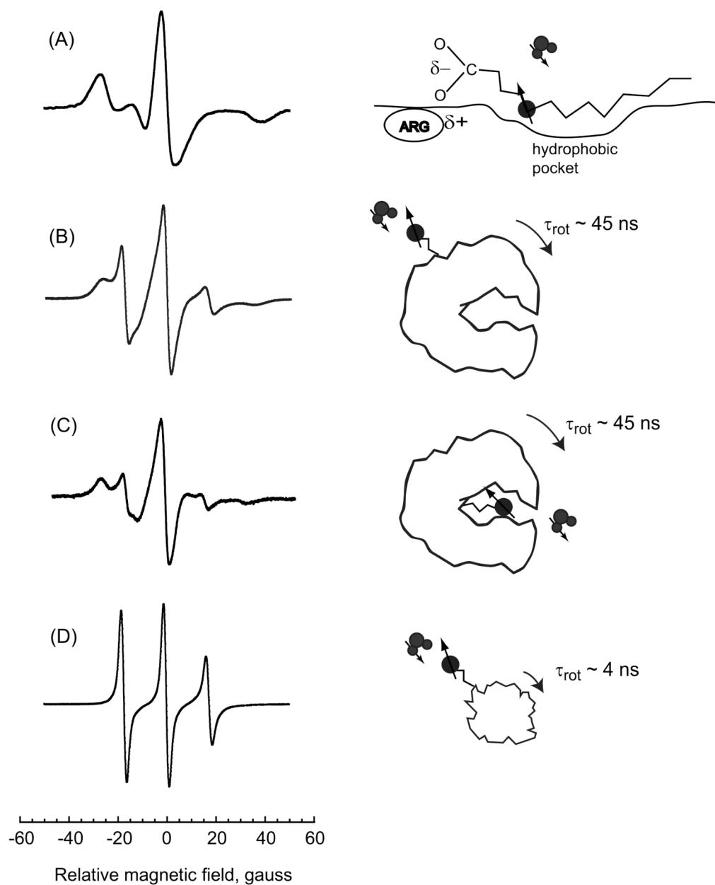
Figure 1. X-band ESR spectra. A) bovine serum albumin with non-covalently bound 5-doxyl steric acid spin-label; B) bovine serum albumin spin-labeled with maleimide-TEMPO covalently bound to cysteine SH; C) bovine serum albumin spin-labeled with maleimide-TEMPO covalently bound to lysine (SH blocked); and D) ribonuclease A spin-labeled with maleimide-TEMPO at lysine.
