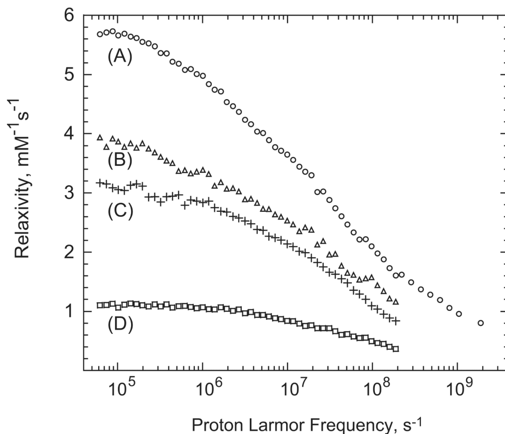
Figure 2. The paramagnetic contribution to the water proton spin-lattice relaxivities as a function of magnetic field strength plotted as the 1 H Larmor frequency at 298 K. A) bovine serum albumin spin-labeled with 5-doxyl stearic acid; B) bovine serum albumin with 1 equivalent of maleimide-TEMPO; C) bovine serum albumin with blocked SH and 1 equivalent of maleimide-TEMPO; D) ribonuclease A spin-labeled with maleimide-TEMPO.
