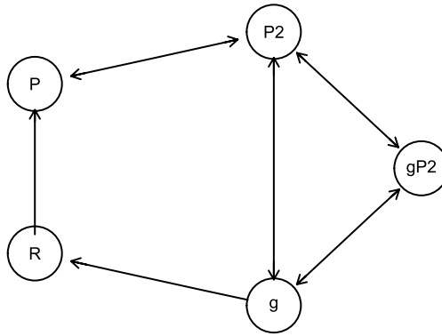
FIG. 1. Kinetic independence graph of the SKM in Example 2.1.
