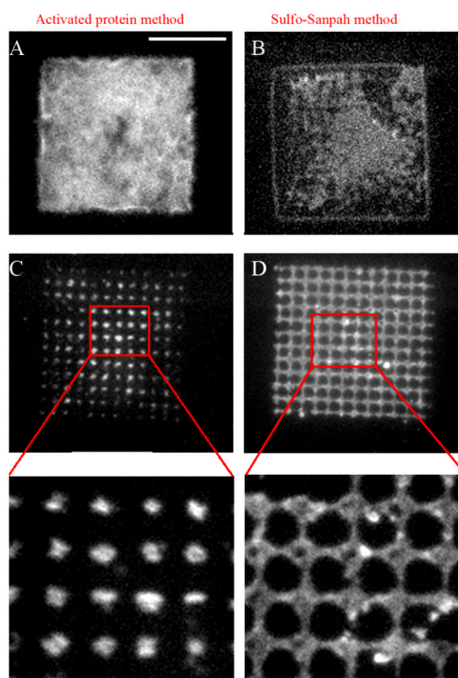
Figure 2. Comparison of protein pattern generated with the present method to that generated by direct microcontact printing on gel surfaces. Fluorescently tagged fibronectin was patterned as 50×50 μm squares using either the present approach (A), or direct microcontact printing on sulfo-SANPAH activated gel surface (B). The present method was able to transfer more protein and cover the adhesive area more completely. It also generated more reproducible patterns and at a higher resolution, as indicated by printing a matrix of 2 μm diameter dots (C, D). Scale bar, 25 μm.
