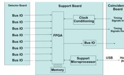
Figure 3. Support Board Block Diagram. This board multiplexes single event words from up to 8 Detector Boards and forwards them to the Coincidence Board. A microprocessor provides communication with the Host PC and control for all of the DBs.
