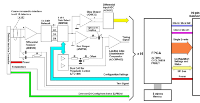
Figure 2. Detector Board Block Diagram. There are 16 independent analog processing chains that digitize an analog input signal and produce a timing signal. These are controlled by a common FPGA that also combines these data (possibly with calibration data that is stored in memory) to determine the gamma ray interaction position, energy, and time. These values are then passed to the next level of electronics via a 96-pin connector.
