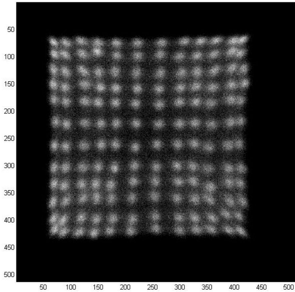
Figure 4. Flood Map from a PET Block Detector Module. The detector module is a 12 \times 12 array of 4 \times 4 \times 22 mm 3 LSO crystals. All 144 crystals are clearly resolved, and the energy resolution for individual crystals is between 10% and 12% fwhm with 511 keV excitation.
