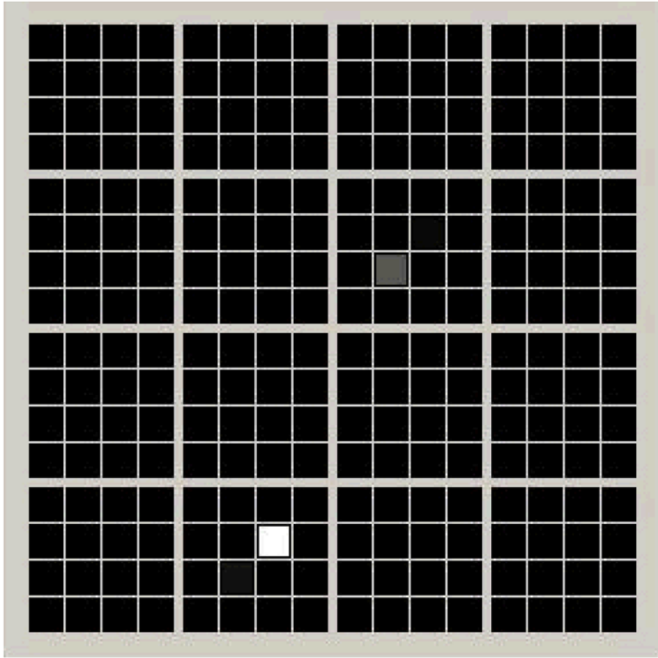
Figure 5. Readout of SiPM Array. A 16 \times 16 array of 3 mm square SiPM elements is read out using a row and column scheme. LSO crystals of different lengths are placed over two of the pixels. The intensity of each pixel in the display is proportional to the event rate in that pixel times the average energy deposited per event. As expected, all but two of the pixels are black, and the pixel with the larger crystal is brighter.
