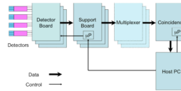
Figure 1. System Architecture. The Detector Boards receive analog input signals and form digital event words. These digital words are multiplexed by the Support Board and by the (optional) Digital Multiplexer Board. Events in time coincidence are identified by the Coincidence Board and sent to the Host PC, which also provides control information.
