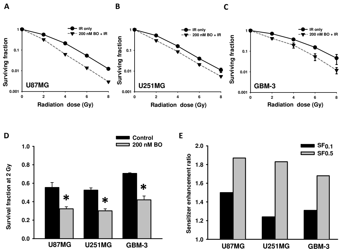
Figure 2 The effect of BO-1051 on tumor cell radiosensitivity. Cultures of (A) U87MG, (B) U251MG and (C) GBM-3 cells were exposed to 200 nM of BO-1051 or DMSO (IR only) for 24 h and irradiated with graded doses of \gamma -rays, rinsed, and fed with fresh growth media. Colony-forming efficiency was determined 10-14 days later, and survival curves were generated after normalizing for cell killing by BO-1051 alone. Points: mean survival fraction from at least 3 independent experiments; bars: SD. (D) The survival fraction after 2 Gy ( SF_2 ), corrected for independent cytotoxic effect of BO-1051, of human glioma cells treated with 200 nM of BO-1051 or control (DMSO) for 24 h pre-radiation was measured. Values are the mean survival fraction \pm SD of at least 3 independent experiments. * p < 0.05 . (E) Sensitizer enhancement ratios (SER) of human glioma cells. SERs were calculated at 10% or 50% cell survival (0.1 or 0.5) by dividing the dose of radiation from the radiation-only surviving curve with the corresponding dose from the BO-1051 plus radiation curve.
