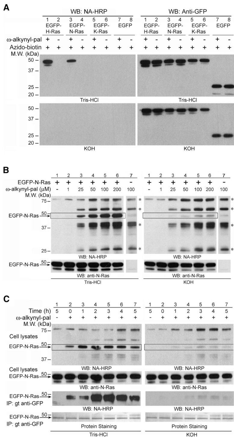
Fig. 4. Incorporation of \omega -alkynyl-palmitate into proteins in COS-7 cells transiently expressing various EGFP-Ras chimeric proteins or EGFP at various label concentrations and time points. A: COS-7 cells transiently expressing EGFP-H-, N-, or K-Ras (lanes 1–6) or EGFP (lanes 7 and 8) were metabolically labeled with 100 \mu M \omega -alkynyl-palmitate or DMSO vehicle as indicated for 3 h followed by solubilization, immunoprecipitation with anti-GFP, and reactions with azido-biotin using click chemistry. B: Lysates (25 \mu g per lane) of COS-7 cells transiently expressing EGFP-N-Ras (lanes 1–6) or without transfection (lane 7) metabolically labeled with increasing concentrations of \omega -alkynyl-palmitate for 3 h. C: Lysates (15 \mu g per lane) of COS-7 cells transiently expressing EGFP-N-Ras metabolically labeled with 100 \mu M \omega -alkynyl-palmitate for various periods of time as shown. Anti-GFP immunoprecipitations corresponding to lanes 1–7 are aligned below the main panels. Of note, for the zero time point (0), the BSA-conjugated \omega -alkynyl-palmitate was added to the media and incubated for 1 min then removed by aspiration. Protein samples were reacted with azido-biotin using click chemistry, separated by electrophoresis, and processed for ECL. Prior to assessment of label incorporation by Western blotting/NA-HRP (1:50,000)/ECL, membranes were incubated in 0.1N Tris-HCl pH 7.0 (upper panels for A and left panels for B and C) or 0.1N KOH (lower panels for A and right panels for B and C). The right panels in A and insets in B and C show the similar expression/immunoprecipitation levels of the EGFP-Ras proteins as assessed by Western blotting using rabbit anti-GFP antibodies or rabbit anti-N-Ras antibodies.
