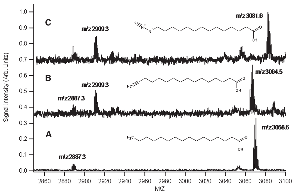
Fig. 3. MALDI time-of-flight mass spectra excerpts of tryptic digests of HMGCS-His6 S-acylated with different palmitate analogs. Following incubation of HMGCS-His 6 with palmitoyl-CoA (A), \omega -alkynyl-palmitoyl-CoA (B), or \omega -azido-tetradecanoyl-CoA (C) alkylation, trypsinization, and reduction, the spectra demonstrate the complete acylation of the peptide containing Cys305 (QAGSDRPFTLDDLQYMIFHTPFCK305 K). Observed m/z values at 3,068.6, 3,064.5, and 3,081.6 are for the acylated peptide containing attached (A) palmitate, (B) alkynyl-palmitate, and (C) azido-palmitate moieties, respectively. The signals at m/z 2,887.3 ( [M+H]^+ ) and m/z 2,909.3 ( [M+Na]^+ ) are from another nonpalmitoylated peptide with sequence GTHMENVYDFYKPNLASEYPIVDGK.
