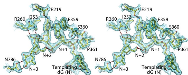
FIGURE 6: Structure of the overhanging 5' template in stereodiagram superimposed onto the final 2F_o - F_c map contoured at 0.5\sigma .
