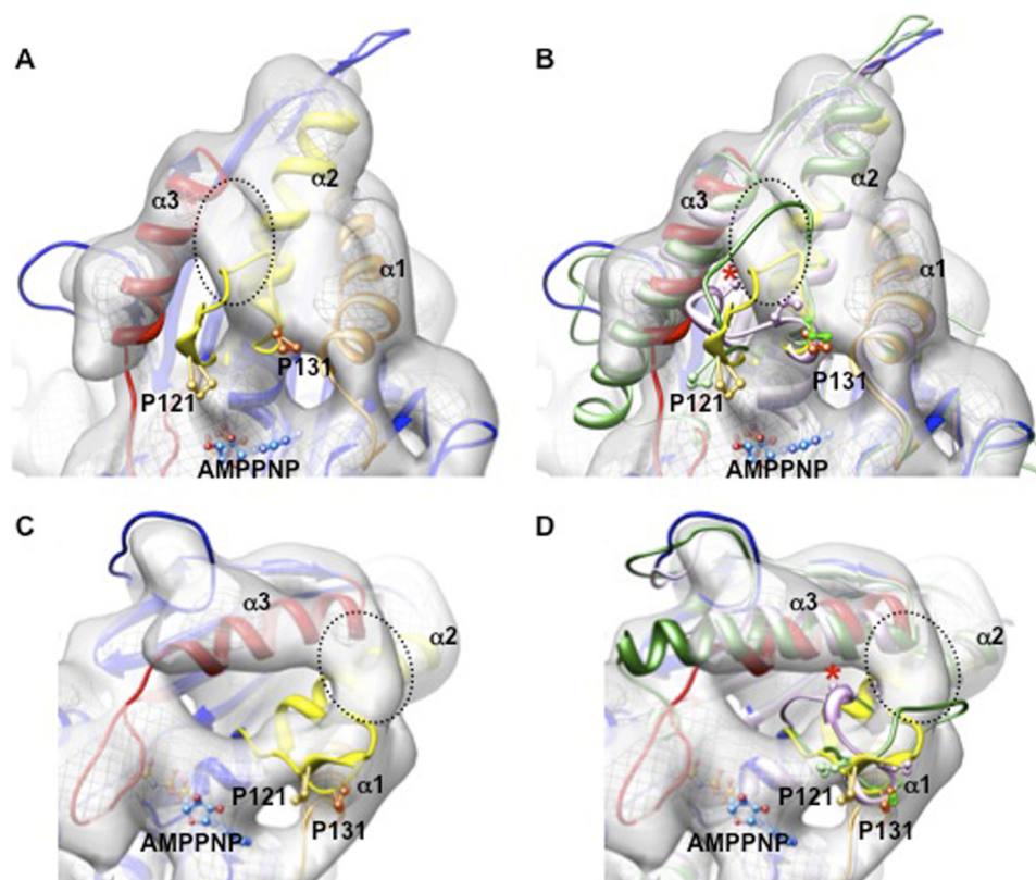
FIGURE 8. Docking of kinesin crystal structures into the cryo-electron microscopy reconstruction of KLP61F ( Drosophila Eg5)-MT complex. A and C , shown are orthogonal views of the docked Eg5-AMPPNP crystal structure which closely matches the cryo-EM density (11) for the length of \alpha 3 (red) and length and orientation of \alpha 4 (not shown). However, L5 protrudes from the cryo-EM structure, and the putative density for the L5 in the MT-bound motor (dotted oval) remains unfilled. B and D , shown are orthogonal views of docked Eg5-AMPPNP crystal structure compared with the Eg5-ADP crystal structure (green (4)) and the Nod-ADP crystal structure (lilac (12)). Note that the position of Pro-131, corresponding to Pro-107 in Nod, is very similar in all of the structures. Pro-121 is in a similar position for Eg5-AMPPNP and Eg5-ADP, whereas the corresponding residue in Nod (Pro-102, indicated by a red asterisk) is positioned toward \alpha 3 , although it also still protrudes from the putative L5 cryo-EM density.
