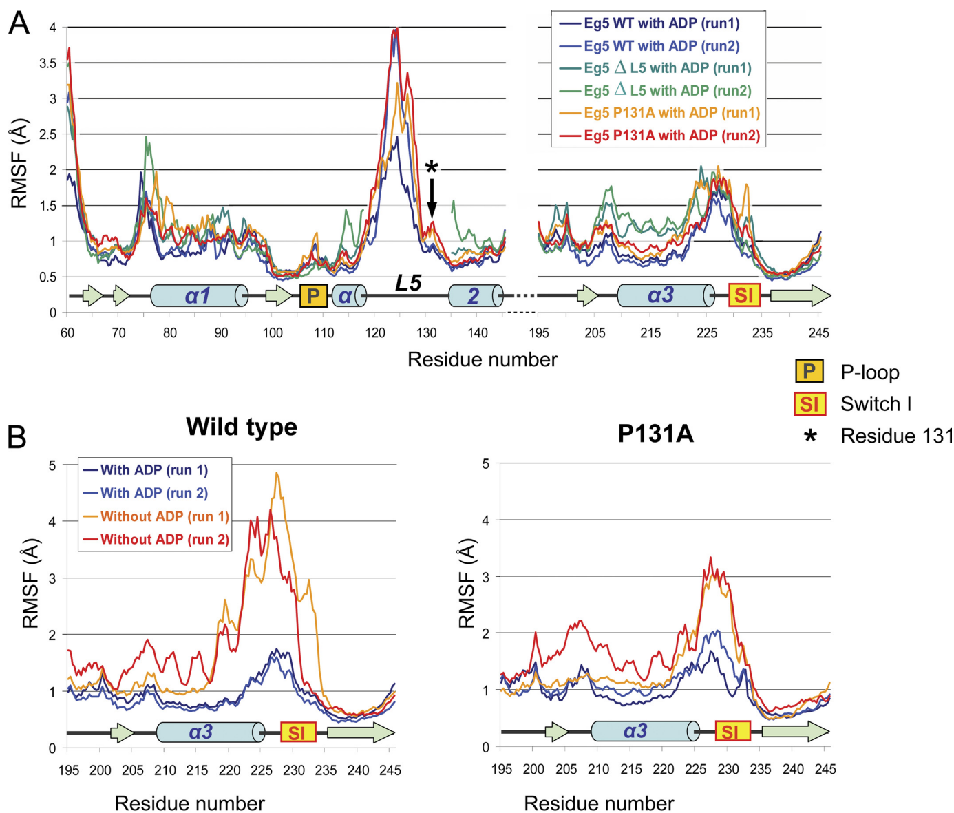
FIGURE 7. r.m.s.f. of the backbone atoms in the region of the \alpha 1 , \alpha 2 , and \alpha 3 helices and surrounding switch I. A , the color code for the different curves is indicated in the top right panel on the graph, and secondary structure elements are represented at the bottom. The P-loop, switch I, and proline 131 are represented as indicated in the legend. The asterisk and arrow denote the location of the P131A mutation. B , shown is the effect of ADP removal on the r.m.s.f. of backbone atoms in the region of the \alpha 3 helix and switch I for Eg5 (left) and the P131A mutant (right). The color code for the different curves is the same in the three graphs and is indicated in the top left panel on the left graph. Secondary structure elements are indicated at the bottom of the graphs.
