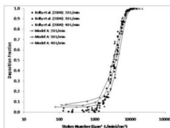
Figure 7. Comparison of particle deposition results from Model A with the experimental data from Kelly et al. (2004b) at inhalation flow rates of 20, 30, and 40 L/min.
