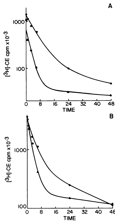
Figure 4. Radioactivity remaining in HDL (A) and plasma (B) after injection of [ 3 H]-cholesteryl ether HDL, shown for a representative pair of animals. CETP-inhibited and control rabbits were injected with ~ 3.5 × 10 6 cpm [ 3 H]cholesteryl ether HDL after the initial infusion of MAb (t = 0). Aliquots of plasma (50 μl) or HDL (200 μl) were counted in duplicate. The results are given as the total counts per minute remaining in plasma or HDL assuming a blood volume of 6% of body weight. Computer generated curves were drawn using a two exponential model of decay (see Methods). ●, TP1 injected animal; ▲, control animal.
