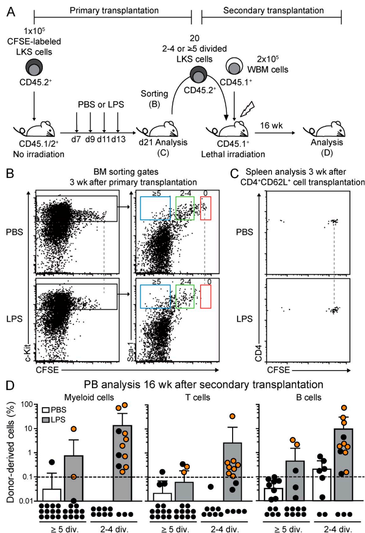
Figure 6. In vivo LPS challenge recruits HSCs into division. (A) Experimental scheme of transplantation and LPS challenge. (B) Representative dot plots gated on donor Lin^- cells from BM of primary transplant recipients at day 21 after transfer of CFSE-labeled LKS cells with or without four injections of LPS. Sorting gates for 0\times - (red), 2-4- (green), or \geq 5\times -divided LKS cells (blue) are shown. Dashed lines represent zero division. (C) Representative dot plots gated on donor CD4^+CD62L^+ cells from spleen of primary transplant recipients at day 21 after transfer of CD4^+CD62L^+ cells with or without four injections of LPS. Dashed lines represent zero division. (D) PB donor engraftment within myeloid, T, and B cells 4 mo after secondary transplantation with 20 2-4- or \geq 5\times -divided LKS cells from PBS- or LPS-treated mice (B). Pooled data from three independent experiments are shown as dots (representing one mouse each) and a bar graph depicting mean \pm SD. Orange dots show the multilineage reconstituted animals. Black dots show animals with one or zero lineages reconstituted. The dashed line at 0.1% shows background threshold set for engraftment cutoff. ND, not detected.
