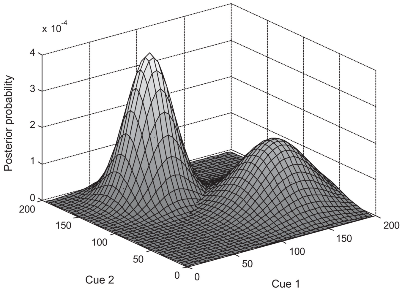
Fig. 4. A two-dimensional MOG with two categories. Each Gaussian is determined by cue-values along both dimensions.
