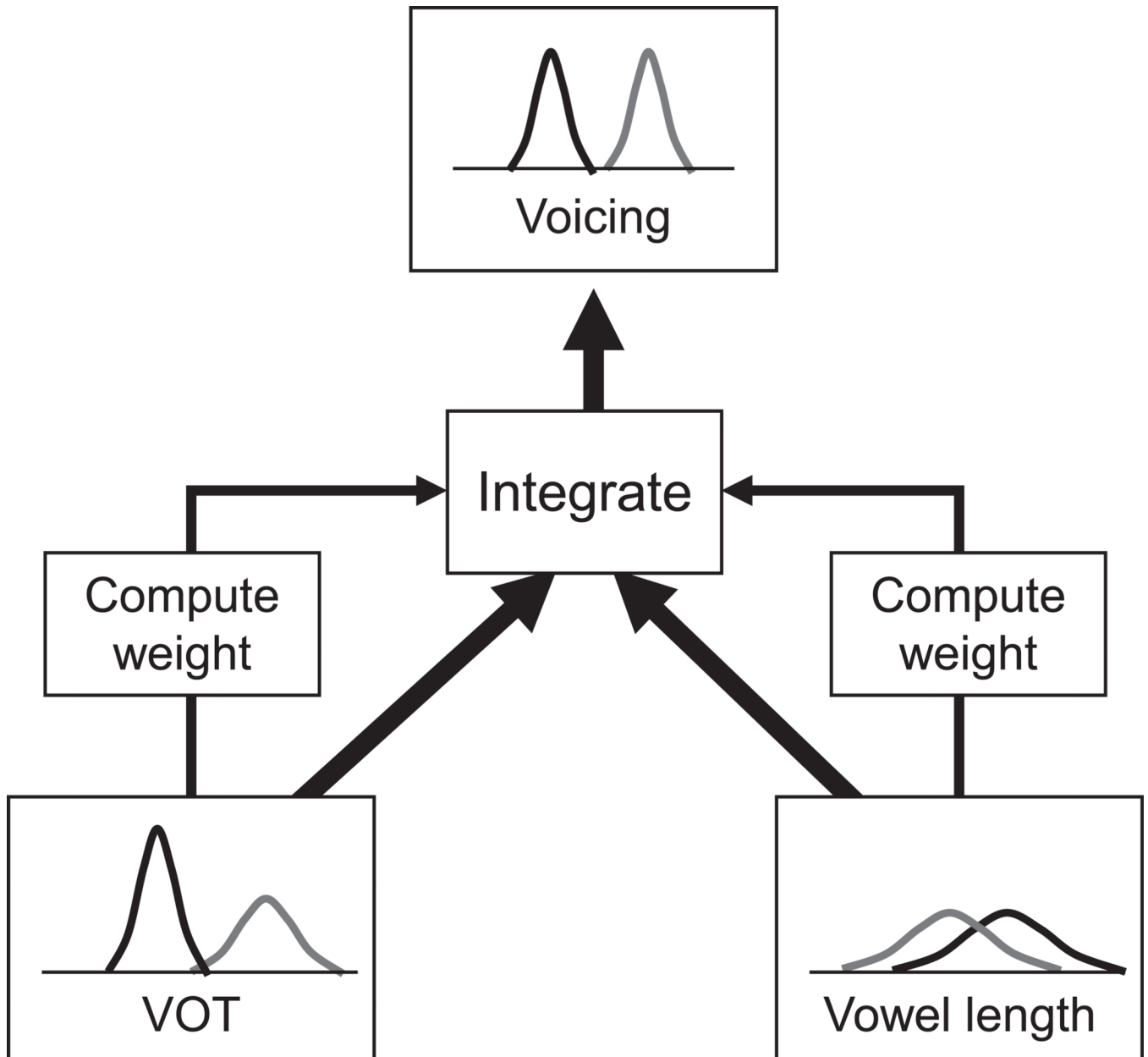
Fig. 3. Schematic representation of the cue-weighting model. Two MOGs receive input for each cue (VOT and VL). The cue weight for each MOG is computed using Equation 5, and the inputs are converted to z-scores. The inputs are then weighted and summed, providing input to a third MOG that reflects voicing categories based on both cues.
