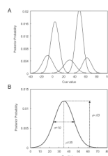
Fig. 2. (A) A mixture of Gaussians (MOG) with five categories along the dimension. (B) Parameters of a Gaussian distribution used in the mixture model. Each distribution is defined by three parameters – its likelihood ( \phi ), its mean ( \mu ), and its standard deviation ( \sigma ).
